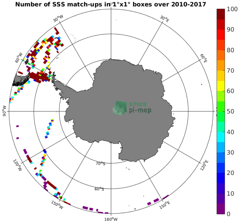
Figure 4: Number of SSS match-ups between TSG (GOSUD-Sailing-ship) SSS and the SMOS SSS L2Q v321 - 0.25 Deg (CATDS-CPDC) SSS product for the Southern Ocean Pi-MEP region over 1°x1° boxes and for the full satellite product period.
