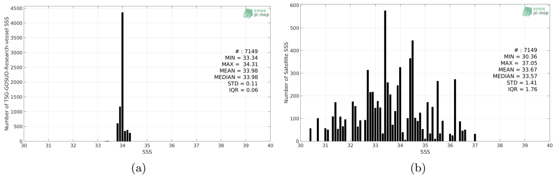
Figure 2: Histograms of SSS from TSG-GOSUD-Research-vessel (a) and SMOS-L3-CATDS-CPDC-V321-L2Q (b) considering all match-up pairs per bins of 0.1 over the Southern Ocean Pi-MEP region and for the full satellite product period.
