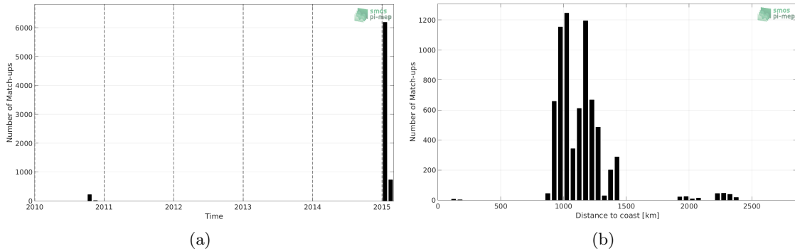
Figure 1: Number of match-ups between TSG-GOSUD-Research-vessel and SMOS-L3-CATDS-CPDC-V321-L2Q SSS as a function of time (a) and as function of the distance to coast (b) over the Southern Ocean Pi-MEP region and for the full satellite product period.
