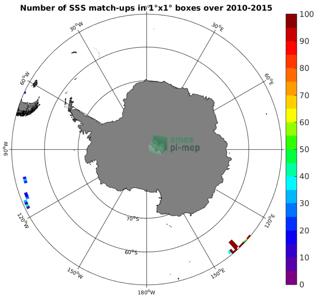
Figure 4: Number of SSS match-ups between TSG-GOSUD-Research-vessel SSS and the SMOS-L3-CATDS-CPDC-V321-L2Q SSS product for the Southern Ocean Pi-MEP region over 1°x1° boxes and for the full satellite product period.
