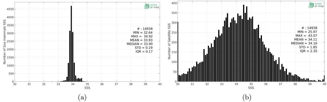
Figure 2: Histograms of SSS from Marine mammals (a) and SMOS SSS L2Q v321 - 0.25 Deg (CATDS-CPDC) (b) considering all match-up pairs per bins of 0.1 over the Southern Ocean Pi-MEP region and for the full satellite product period.
