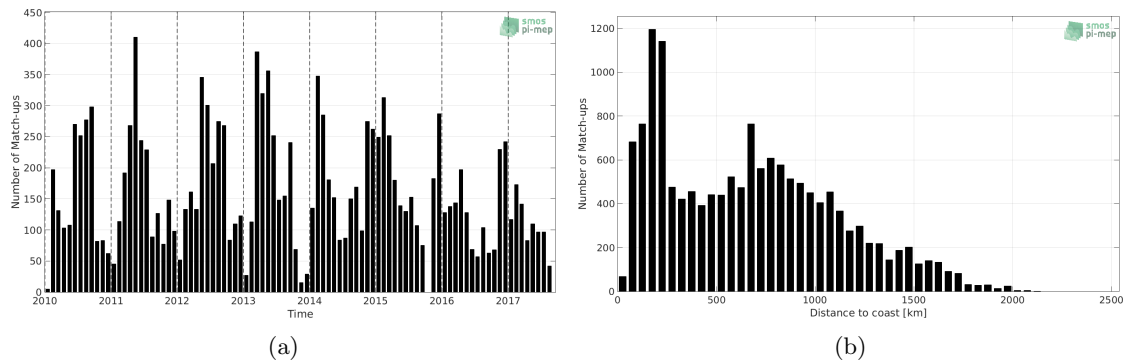
Figure 1: Number of match-ups between Marine mammals and SMOS SSS L2Q v321 - 0.25 Deg (CATDS-CPDC) SSS as a function of time (a) and as function of the distance to coast (b) over the Southern Ocean Pi-MEP region and for the full satellite product period.
