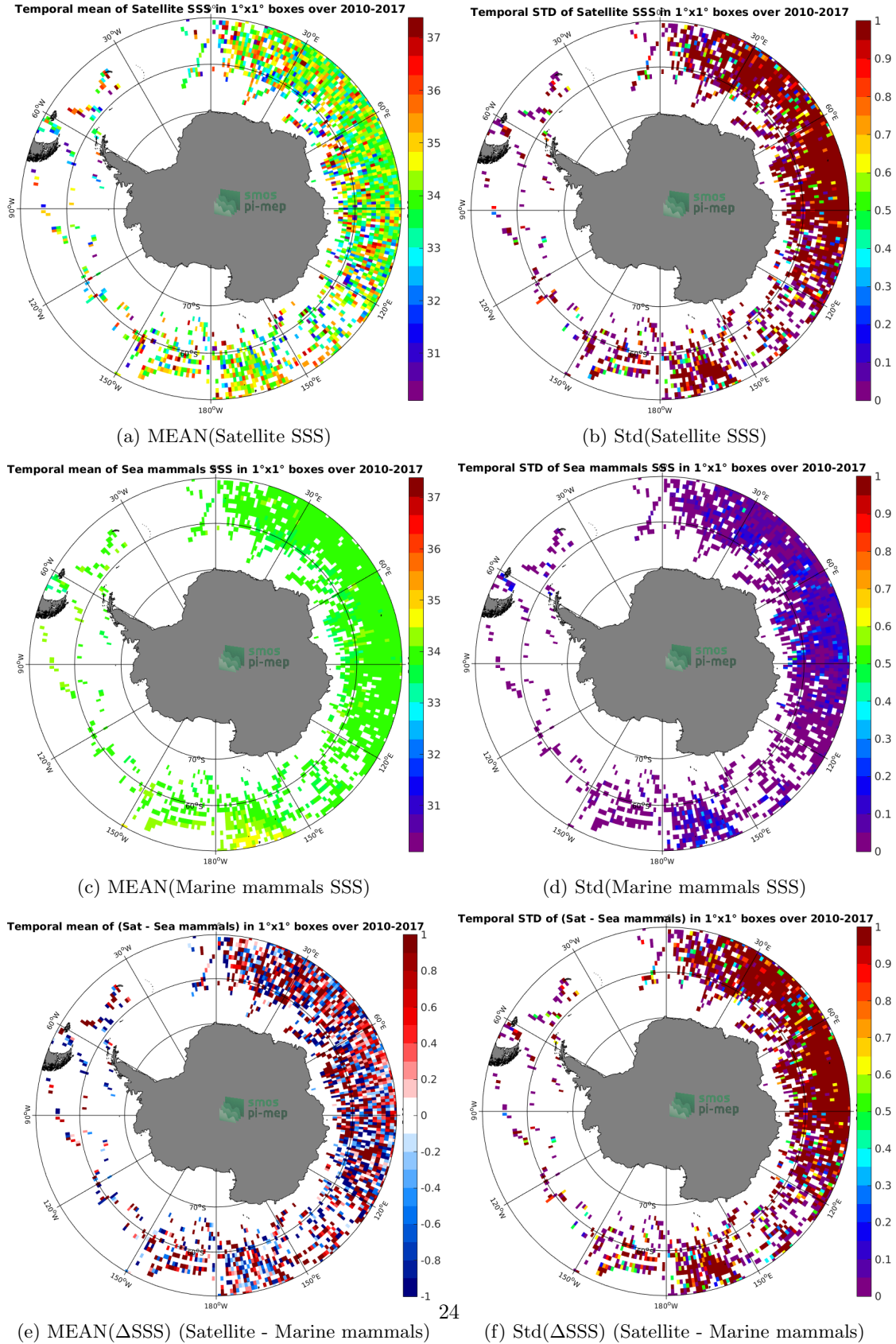
Figure 6: Temporal mean (left) and Std (right) of SSS from SMOS SSS L2Q v321 - 0.25 Deg (CATDS-CPDC) (top), Marine mammals (middle), and of \Delta SSS (Satellite - Marine mammals). Only match-up pairs are used to generate these maps.
