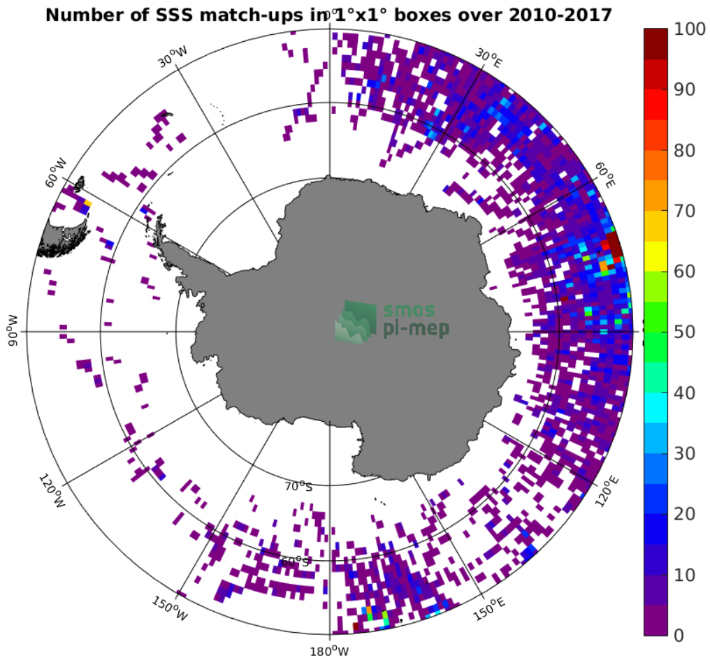
Figure 4: Number of SSS match-ups between Marine mammals SSS and the SMOS SSS L2Q v321 - 0.25 Deg (CATDS-CPDC) SSS product for the Southern Ocean Pi-MEP region over 1^\circ \times 1^\circ boxes and for the full satellite product period.
