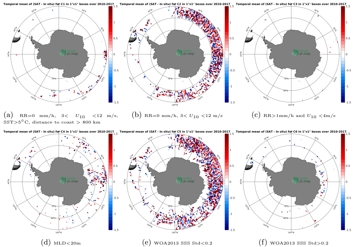
Figure 12: Temporal mean gridded over spatial boxes of size 1^{\circ}\times 1^{\circ} of \Delta\text{SSS} (SMOS SSS L2Q v321 - 0.25 Deg (CATDS-CPDC) - Marine mammals) for 6 different subdatasets corresponding to:RR=0 mm/h, 3 < U_{10} < 12 m/s, SST >5^{\circ}\text{C} , distance to coast > 800 km (a), RR=0 mm/h, 3 < U_{10} < 12 m/s (b), RR >1 mm/h and U_{10} < 4 m/s (c),MLD <20 m (d),WOA2013 SSS Std <0.2 (e),WOA2013 SSS Std >0.2 (f).
