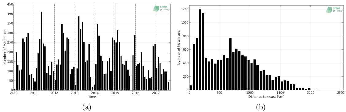
Figure 1: Number of match-ups between Sea mammals and SMOS SSS L2Q v321 - 0.25 Deg (CATDS-CPDC) SSS as a function of time (a) and as function of the distance to coast (b) over the Southern Ocean Pi-MEP region and for the full satellite product period.
