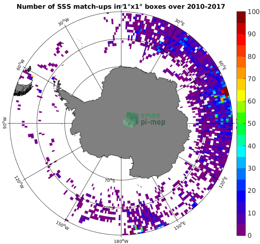
Figure 4: Number of SSS match-ups between Sea mammals SSS and the SMOS SSS L2Q v321 - 0.25 Deg (CATDS-CPDC) SSS product for the Southern Ocean Pi-MEP region over 1^{\circ} \times 1^{\circ} boxes and for the full satellite product period.
