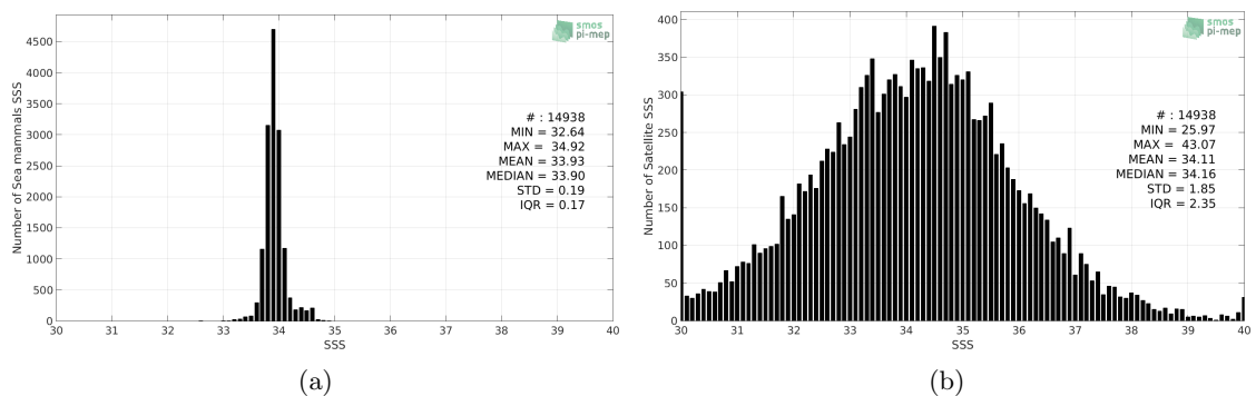
Figure 2: Histograms of SSS from Sea mammals (a) and SMOS SSS L2Q v321 - 0.25 Deg (CATDS-CPDC) (b) considering all match-up pairs per bins of 0.1 over the Southern Ocean Pi-MEP region and for the full satellite product period.
