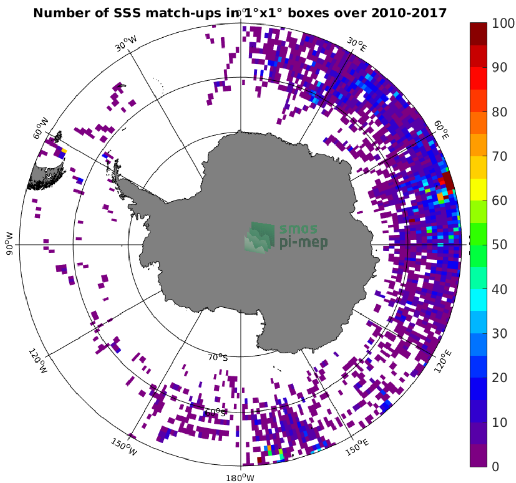
Figure 4: Number of SSS match-ups between Sea mammals SSS and the SMOS SSS L2Q v321 - 0.25 Deg (CATDS-CPDC) SSS product for the Southern Ocean Pi-MEP region over 1°x1° boxes and for the full satellite product period.
