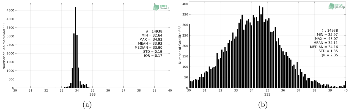
Figure 2: Histograms of SSS from Sea mammals (a) and SMOS L2Q v321 - 0.25 Deg (CATDS-CPDC) (b) considering all match-up pairs per bins of 0.1 over the Southern Ocean Pi-MEP region and for the full satellite product period.
