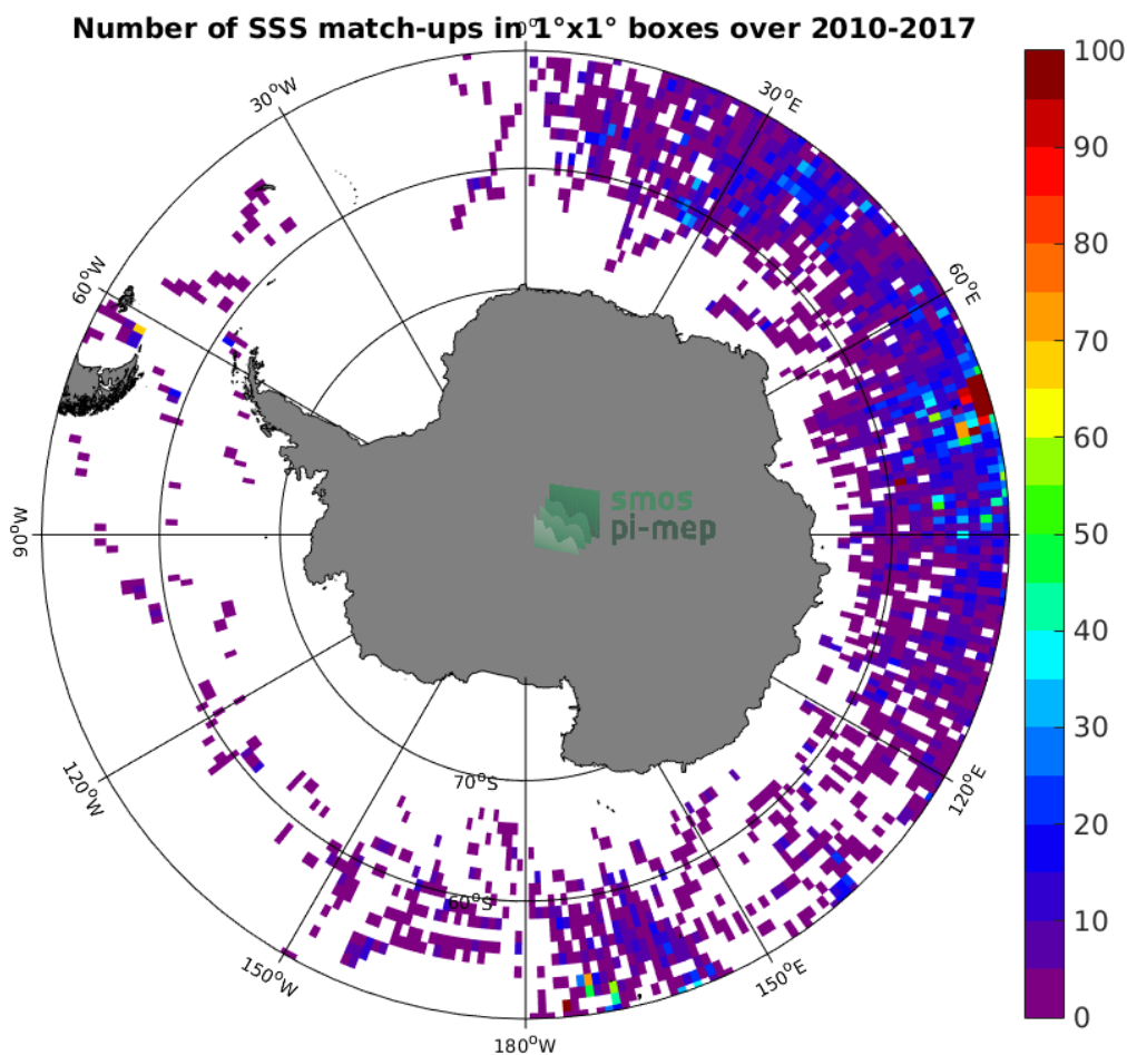
Figure 4: Number of SSS match-ups between Sea mammals SSS and the SMOS L2Q v321 - 0.25 Deg (CATDS-CPDC) SSS product for the Southern Ocean Pi-MEP region over 1°x1° boxes and for the full satellite product period.
