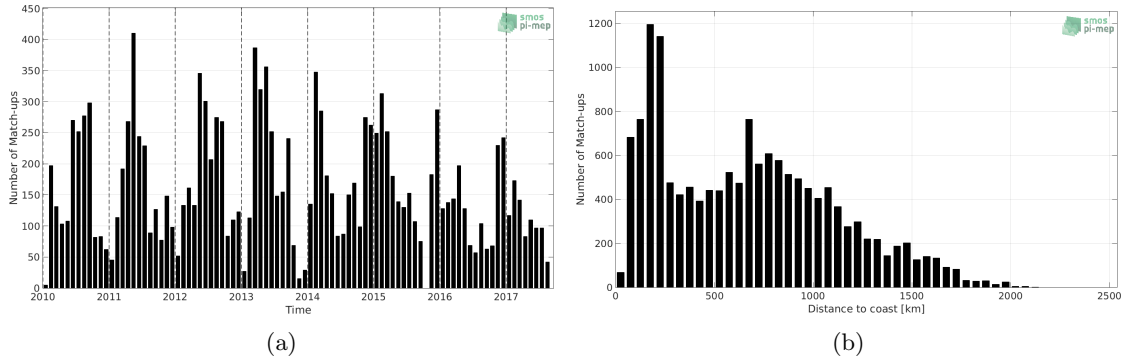
Figure 1: Number of match-ups between Sea mammals and SMOS L2Q v321 - 0.25 Deg (CATDS-CPDC) SSS as a function of time (a) and as function of the distance to coast (b) over the Southern Ocean Pi-MEP region and for the full satellite product period.
