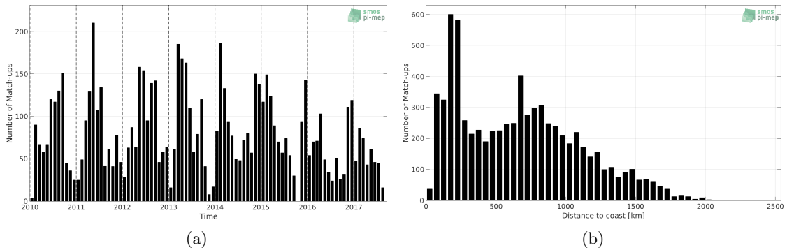
Figure 1: Number of match-ups between Sea mammals and SMOS-L3-CATDS-CPDC-V321-L2Q SSS as a function of time (a) and as function of the distance to coast (b) over the Southern Ocean Pi-MEP region and for the full satellite product period.
