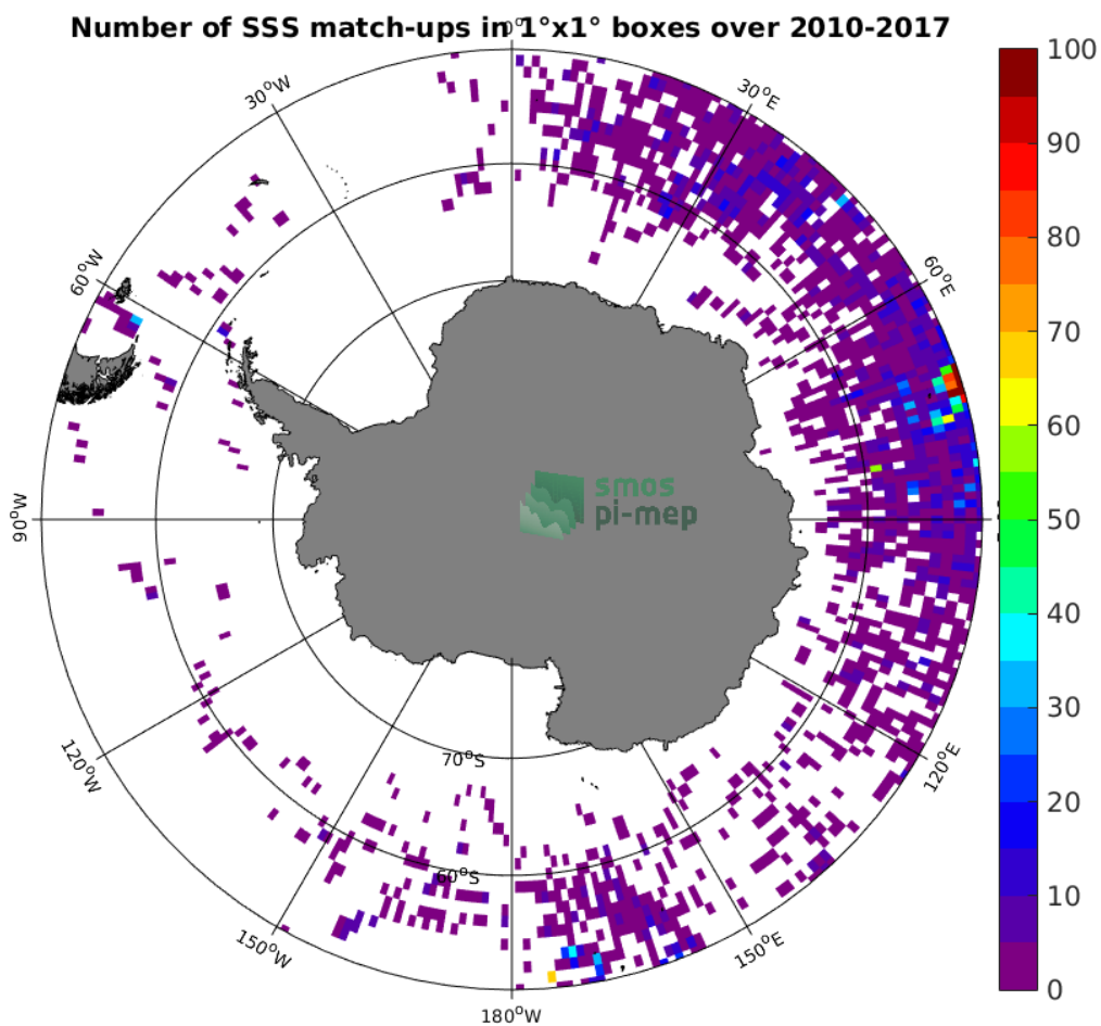
Figure 4: Number of SSS match-ups between Sea mammals SSS and the SMOS-L3-CATDS-CPDC-V321-L2Q SSS product for the Southern Ocean Pi-MEP region over 1^{\circ} \times 1^{\circ} boxes and for the full satellite product period.
