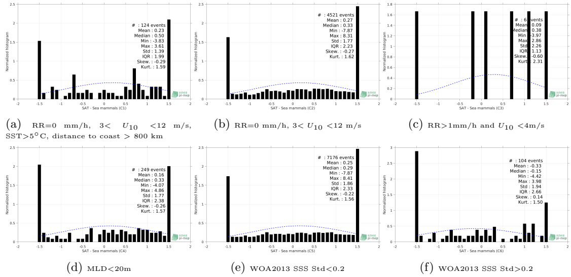
Figure 13: Normalized histogram of \Delta SSS (SMOS-L3-CATDS-CPDC-V321-L2Q - Sea mammals) for 6 different subdatasets corresponding to: RR=0 mm/h, 3 < U_{10} < 12 m/s, SST>5°C, distance to coast > 800 km (a), RR=0 mm/h, 3 < U_{10} < 12 m/s (b), RR>1mm/h and U_{10} < 4 m/s (c), MLD<20m (d), WOA2013 SSS Std<0.2 (e), WOA2013 SSS Std>0.2 (f).
