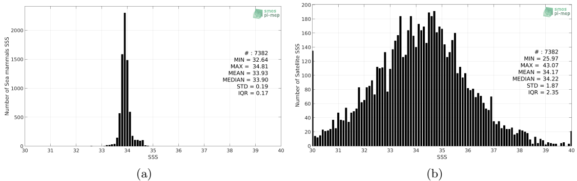
Figure 2: Histograms of SSS from Sea mammals (a) and SMOS-L3-CATDS-CPDC-V321-L2Q (b) considering all match-up pairs per bins of 0.1 over the Southern Ocean Pi-MEP region and for the full satellite product period.
