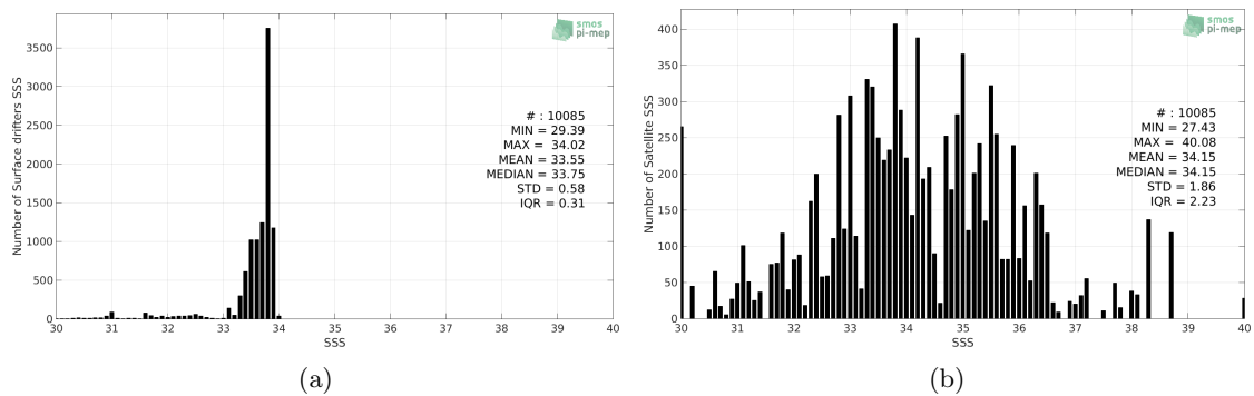
Figure 2: Histograms of SSS from Surface drifters (a) and SMOS L2Q v321 - 0.25 Deg (CATDS-CPDC) (b) considering all match-up pairs per bins of 0.1 over the Southern Ocean Pi-MEP region and for the full satellite product period.
