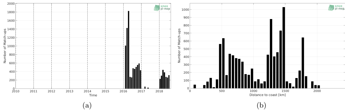
Figure 1: Number of match-ups between Surface drifters and SMOS L2Q v321 - 0.25 Deg (CATDS-CPDC) SSS as a function of time (a) and as function of the distance to coast (b) over the Southern Ocean Pi-MEP region and for the full satellite product period.
