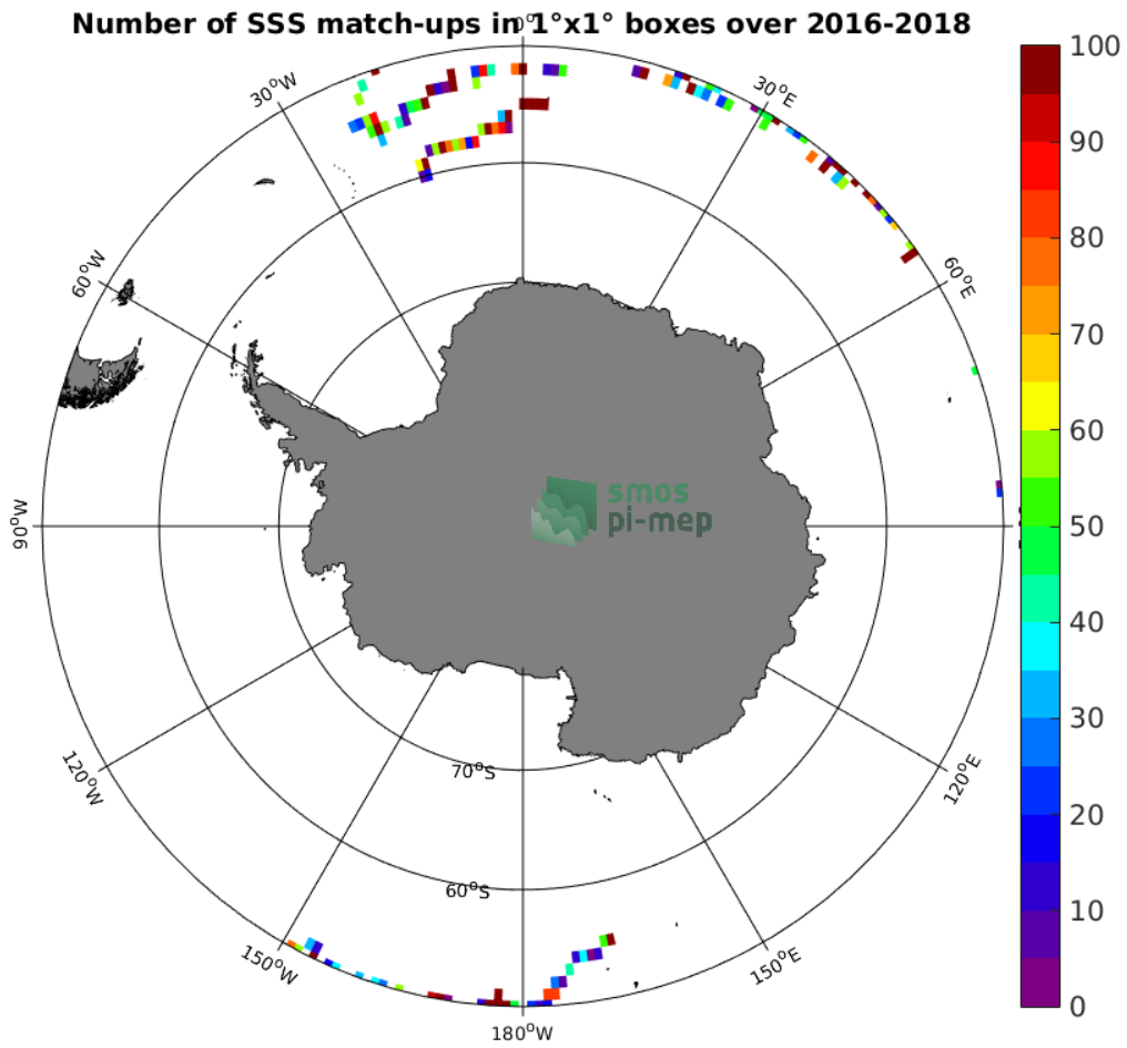
Figure 3: Number of SSS match-ups between Surface drifters SSS and the SMOS L2Q v321 - 0.25 Deg (CATDS-CPDC) SSS product for the Southern Ocean Pi-MEP region over 1°x1° boxes and for the full satellite product period.
