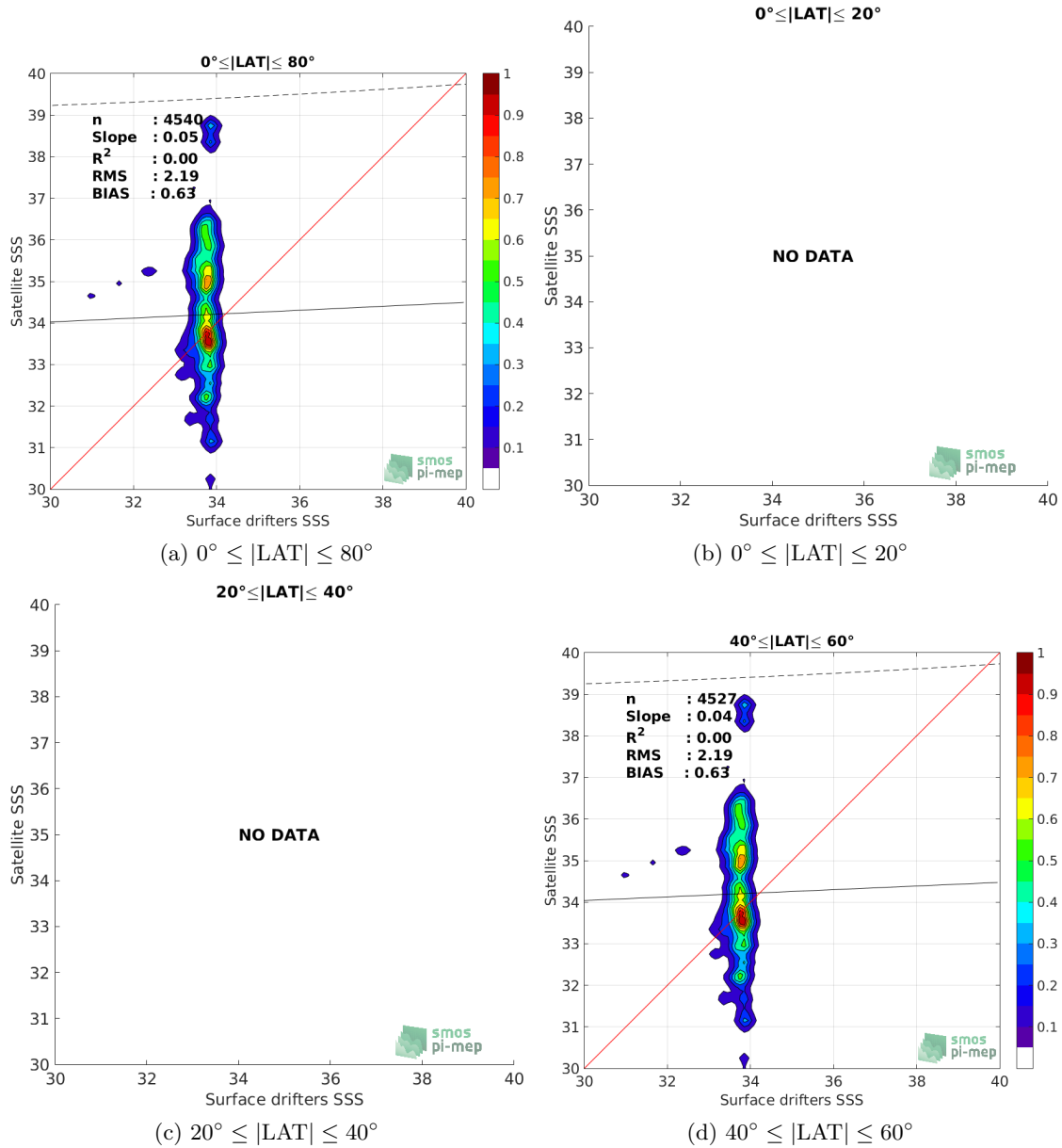
Figure 8: Contour maps of the concentration of SMOS-L3-CATDS-CPDC-V321-L2Q SSS (y-axis) versus Surface drifters SSS (x-axis) at match-up pairs for different latitude bands. For each plot, the red line shows x=y . The black thin and dashed lines indicate a linear fit through the data cloud and the \pm 95\% confidence levels, respectively. The number match-up pairs n , the slope and R^2 coefficient of the linear fit, the root mean square (RMS) and the mean bias between satellite and in situ data are indicated for each latitude band in each plots.
