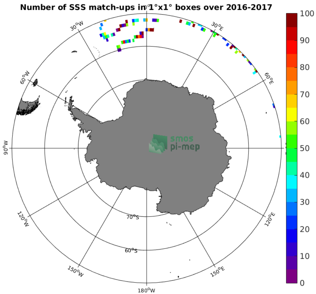
Figure 3: Number of SSS match-ups between Surface drifters SSS and the SMOS-L3-CATDS-CPDC-V321-L2Q SSS product for the Southern Ocean Pi-MEP region over 1^\circ \times 1^\circ boxes and for the full satellite product period.
