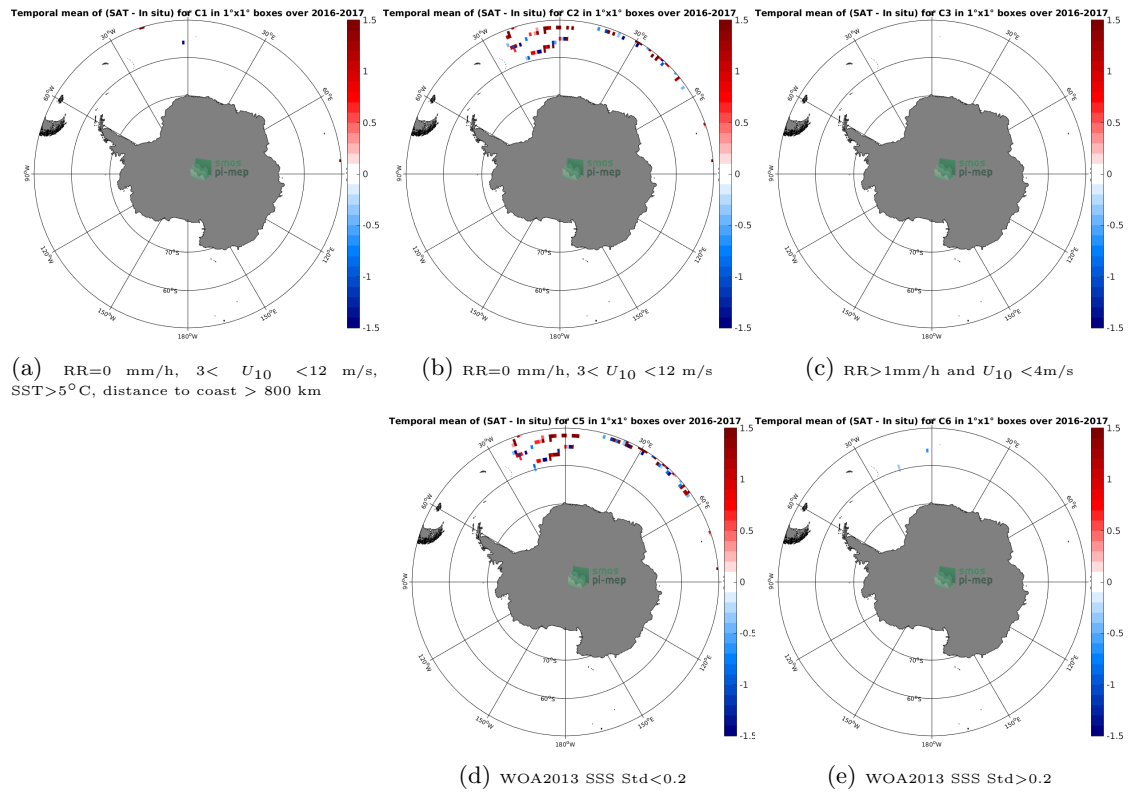
Figure 11: Temporal mean gridded over spatial boxes of size 1^\circ \times 1^\circ of \Delta SSS (SMOS-L3-CATDS-CPDC-V321-L2Q - Surface drifters) for 5 different subdatasets corresponding to:RR=0 mm/h, 3 < U_{10} < 12 m/s, SST >5^\circ C, distance to coast > 800 km (a), RR=0 mm/h, 3 < U_{10} < 12 m/s (b), RR >1 mm/h and U_{10} < 4 m/s (c), WOA2013 SSS Std <0.2 (d), WOA2013 SSS Std >0.2 (e).
