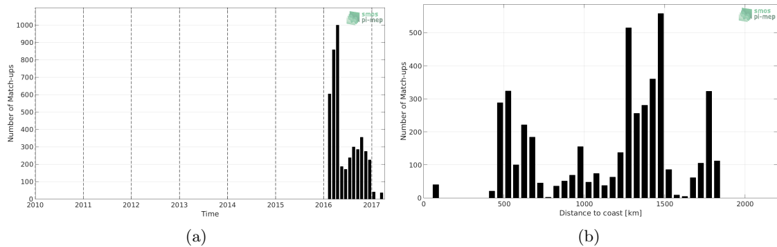
Figure 1: Number of match-ups between Surface drifters and SMOS-L3-CATDS-CPDC-V321-L2Q SSS as a function of time (a) and as function of the distance to coast (b) over the Southern Ocean Pi-MEP region and for the full satellite product period.
