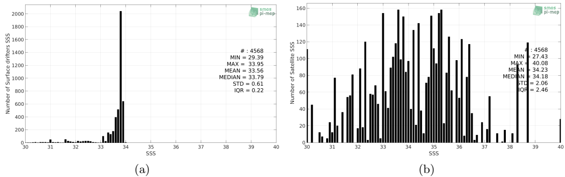
Figure 2: Histograms of SSS from Surface drifters (a) and SMOS-L3-CATDS-CPDC-V321-L2Q (b) considering all match-up pairs per bins of 0.1 over the Southern Ocean Pi-MEP region and for the full satellite product period.
