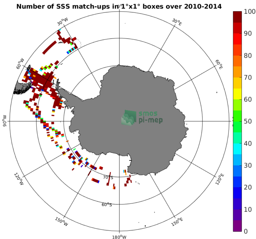
Figure 4: Number of SSS match-ups between TSG (SAMOS) SSS and the SMOS SSS L3 v317 - Monthly - 25 km (CATDS-CPDC) SSS product for the Southern Ocean Pi-MEP region over 1°x1° boxes and for the full satellite product period.
