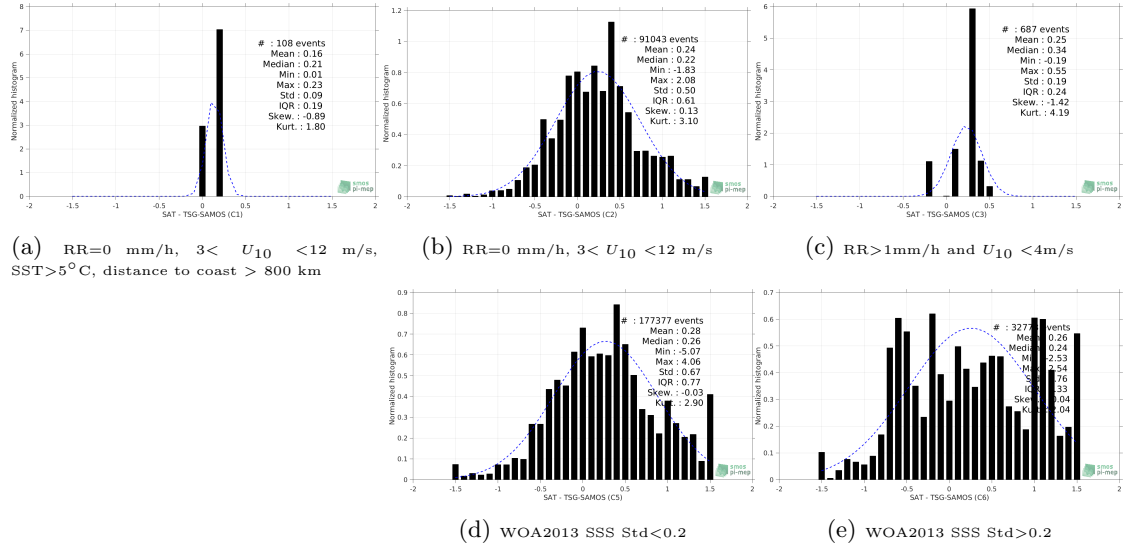
Figure 13: Normalized histogram of \Delta SSS (SMOS L3 v317 - Monthly - 25 km (CATDS-CPDC) - TSG-SAMOS) for 5 different subdatasets corresponding to: RR=0 mm/h, 3 < U_{10} < 12 m/s, SST>5°C, distance to coast > 800 km (a), RR=0 mm/h, 3 < U_{10} < 12 m/s (b), RR>1mm/h and U_{10} < 4 m/s (c), WOA2013 SSS Std<0.2 (d), WOA2013 SSS Std>0.2 (e).
