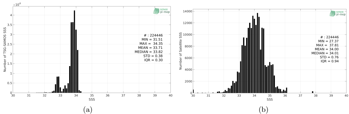
Figure 2: Histograms of SSS from TSG-SAMOS (a) and SMOS L3 v317 - Monthly - 25 km (CATDS-CPDC) (b) considering all match-up pairs per bins of 0.1 over the Southern Ocean Pi-MEP region and for the full satellite product period.
