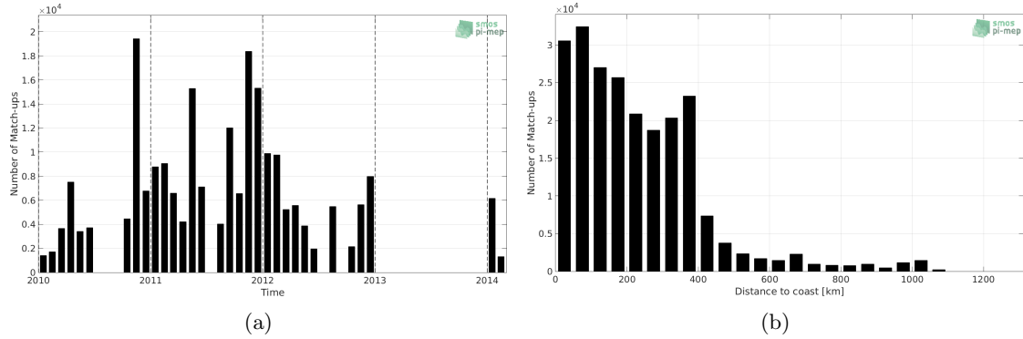
Figure 1: Number of match-ups between TSG-SAMOS and SMOS L3 v317 - Monthly - 25 km (CATDS-CPDC) SSS as a function of time (a) and as function of the distance to coast (b) over the Southern Ocean Pi-MEP region and for the full satellite product period.
