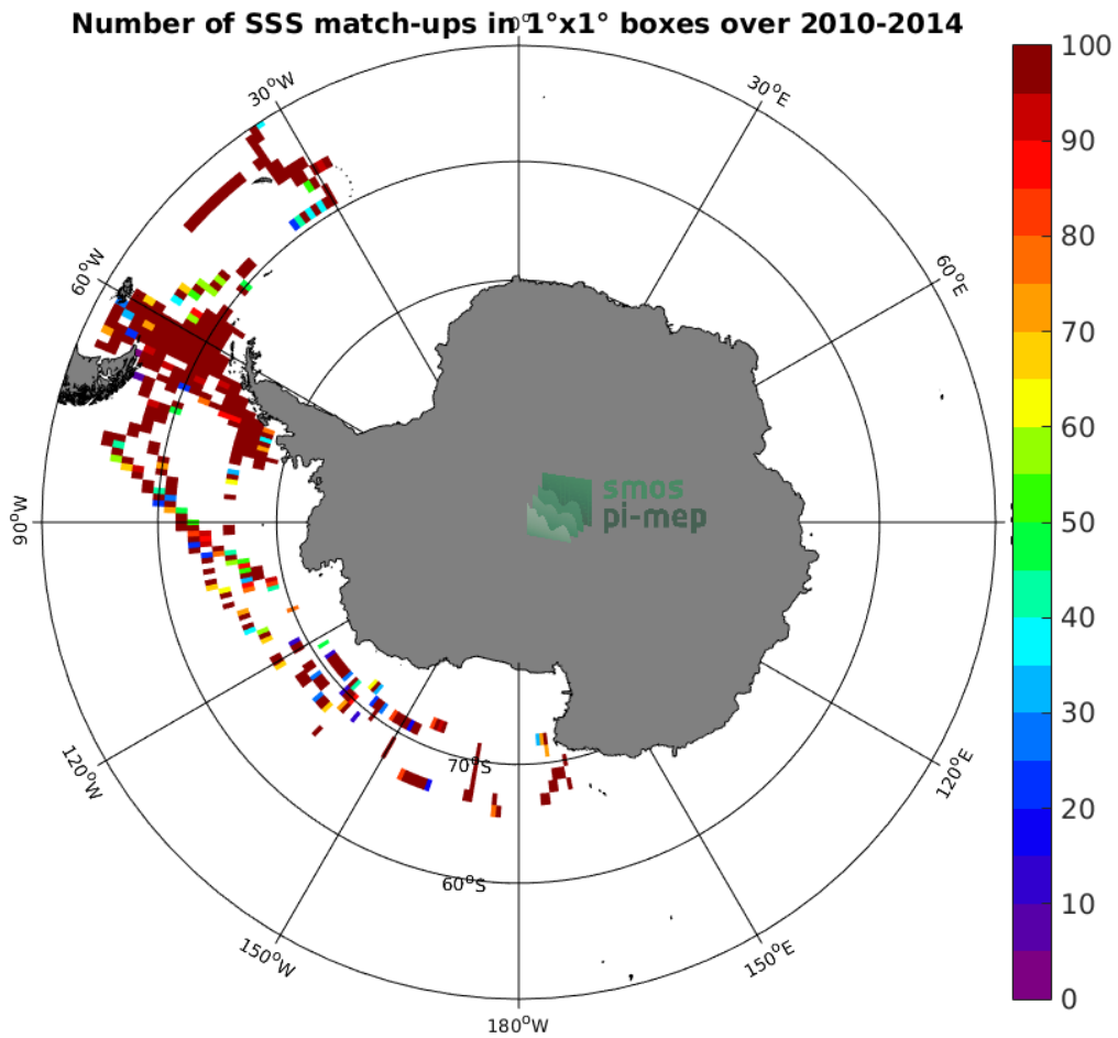
Figure 4: Number of SSS match-ups between TSG-SAMOS SSS and the SMOS L3 v317 - Monthly - 25 km (CATDS-CPDC) SSS product for the Southern Ocean Pi-MEP region over 1°x1° boxes and for the full satellite product period.
