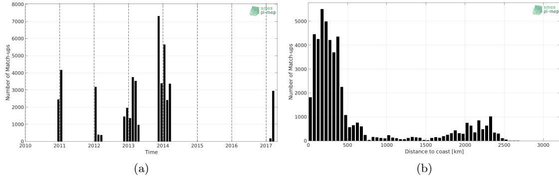
Figure 1: Number of match-ups between TSG-GOSUD-Sailing-ship and SMOS L3 v317 - Monthly - 25 km (CATDS-CPDC) SSS as a function of time (a) and as function of the distance to coast (b) over the Southern Ocean Pi-MEP region and for the full satellite product period.
