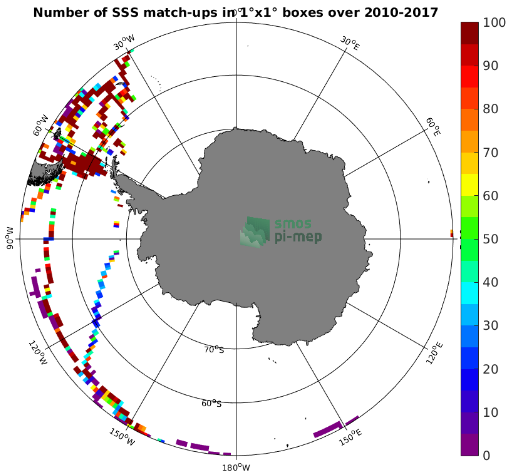
Figure 4: Number of SSS match-ups between TSG-GOSUD-Sailing-ship SSS and the SMOS L3 v317 - Monthly - 25 km (CATDS-CPDC) SSS product for the Southern Ocean Pi-MEP region over 1^\circ \times 1^\circ boxes and for the full satellite product period.
