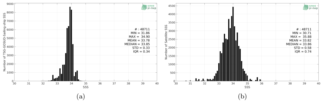
Figure 2: Histograms of SSS from TSG-GOSUD-Sailing-ship (a) and SMOS L3 v317 - Monthly - 25 km (CATDS-CPDC) (b) considering all match-up pairs per bins of 0.1 over the Southern Ocean Pi-MEP region and for the full satellite product period.
