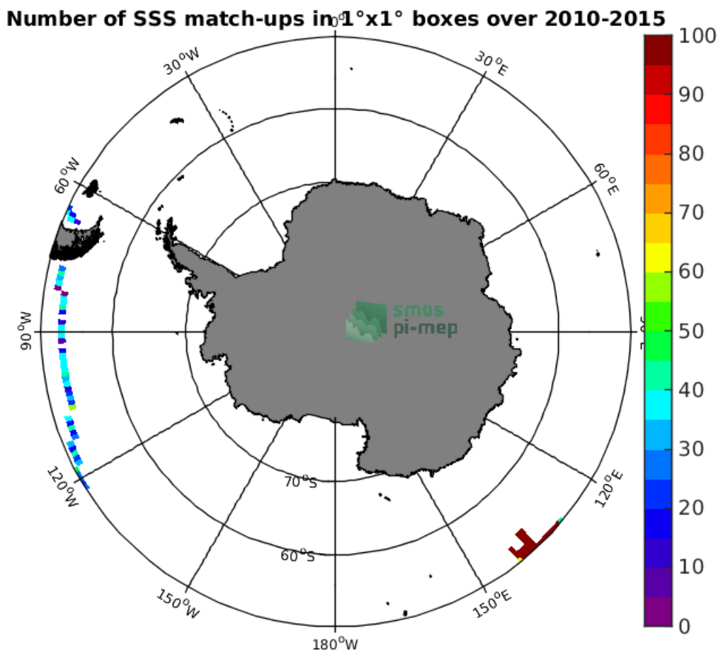
Figure 4: Number of SSS match-ups between TSG-GOSUD-Research-vessel SSS and the SMOS-L3-CATDS-CPDC-V317-MONTHLY-25KM SSS product for the Southern Ocean Pi-MEP region over 1°x1° boxes and for the full satellite product period.
