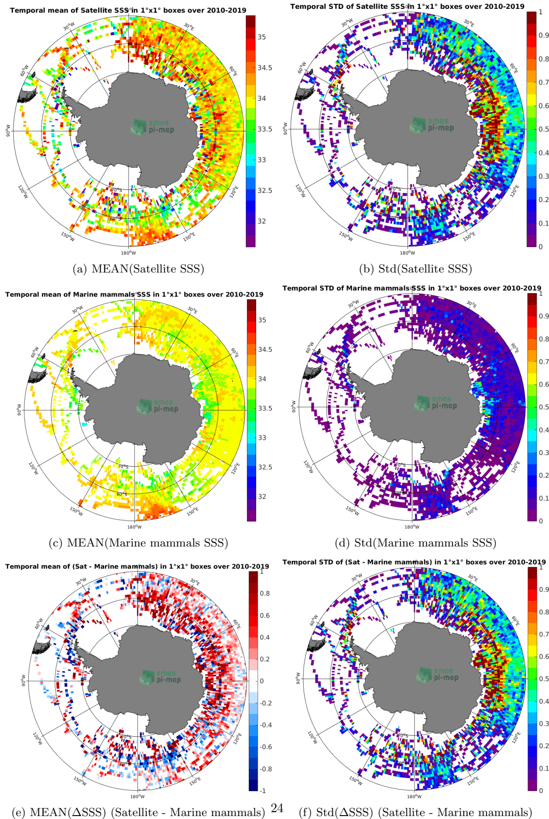
Figure 6: Temporal mean (left) and Std (right) of SSS from SMOS SSS L3 v317 - Monthly - 25 km (CATDS-CPDC) (top), Marine mammals (middle), and of \Delta SSS (Satellite - Marine mammals). Only match-up pairs are used to generate these maps.
