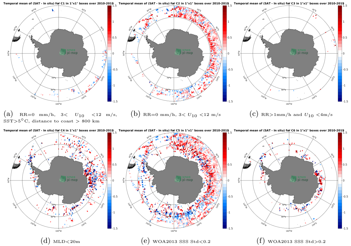
Figure 12: Temporal mean gridded over spatial boxes of size 1^{\circ} \times 1^{\circ} of \Delta\text{SSS} (SMOS SSS L3 v317 - Monthly - 25 km (CATDS-CPDC) - Marine mammals) for 6 different subdatasets corresponding to: RR=0 mm/h, 3 < U_{10} < 12 m/s, SST >5^{\circ}\text{C} , distance to coast > 800 km (a), RR=0 mm/h, 3 < U_{10} < 12 m/s (b), RR >1 mm/h and U_{10} < 4 m/s (c),MLD <20 m (d),WOA2013 SSS Std <0.2 (e),WOA2013 SSS Std >0.2 (f).
