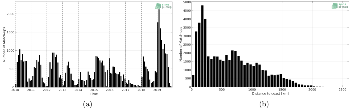
Figure 1: Number of match-ups between Marine mammals and SMOS SSS L3 v317 - Monthly - 25 km (CATDS-CPDC) SSS as a function of time (a) and as function of the distance to coast (b) over the Southern Ocean Pi-MEP region and for the full satellite product period.
