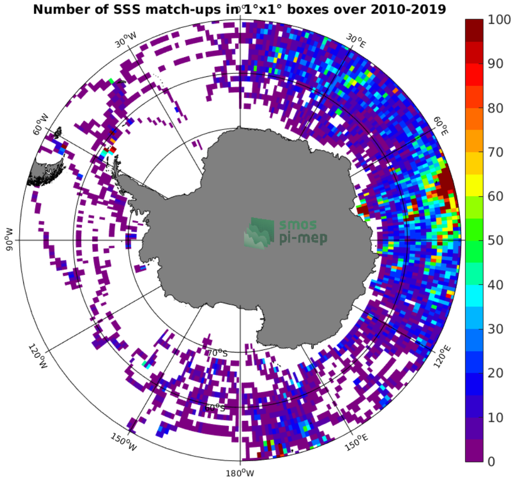
Figure 4: Number of SSS match-ups between Marine mammals SSS and the SMOS SSS L3 v317 - Monthly - 25 km (CATDS-CPDC) SSS product for the Southern Ocean Pi-MEP region over 1^\circ \times 1^\circ boxes and for the full satellite product period.
