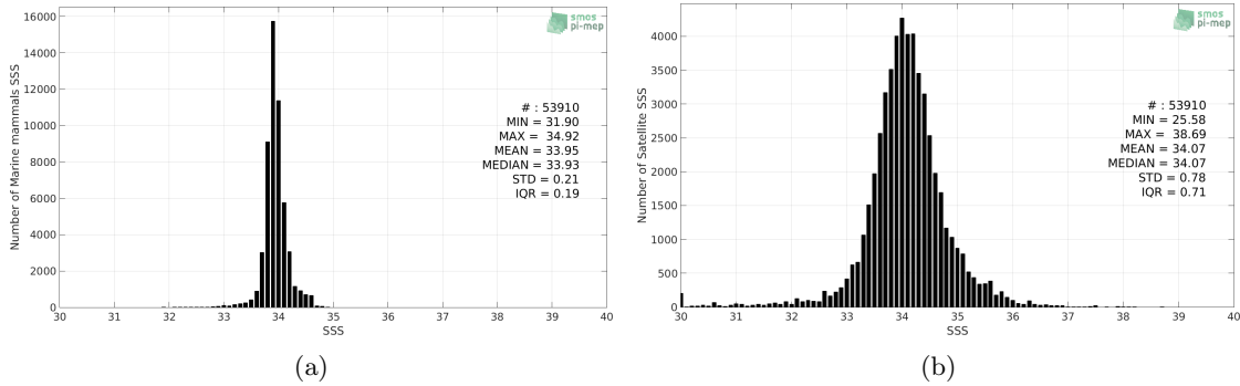
Figure 2: Histograms of SSS from Marine mammals (a) and SMOS SSS L3 v317 - Monthly - 25 km (CATDS-CPDC) (b) considering all match-up pairs per bins of 0.1 over the Southern Ocean Pi-MEP region and for the full satellite product period.
