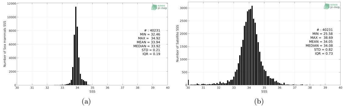
Figure 2: Histograms of SSS from Sea mammals (a) and SMOS SSS L3 v317 - Monthly - 25 km (CATDS-CPDC) (b) considering all match-up pairs per bins of 0.1 over the Southern Ocean Pi-MEP region and for the full satellite product period.
