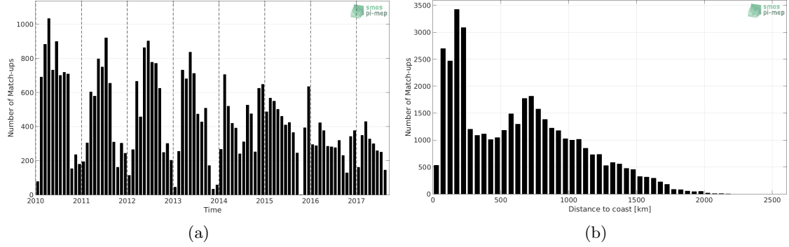
Figure 1: Number of match-ups between Sea mammals and SMOS SSS L3 v317 - Monthly - 25 km (CATDS-CPDC) SSS as a function of time (a) and as function of the distance to coast (b) over the Southern Ocean Pi-MEP region and for the full satellite product period.
