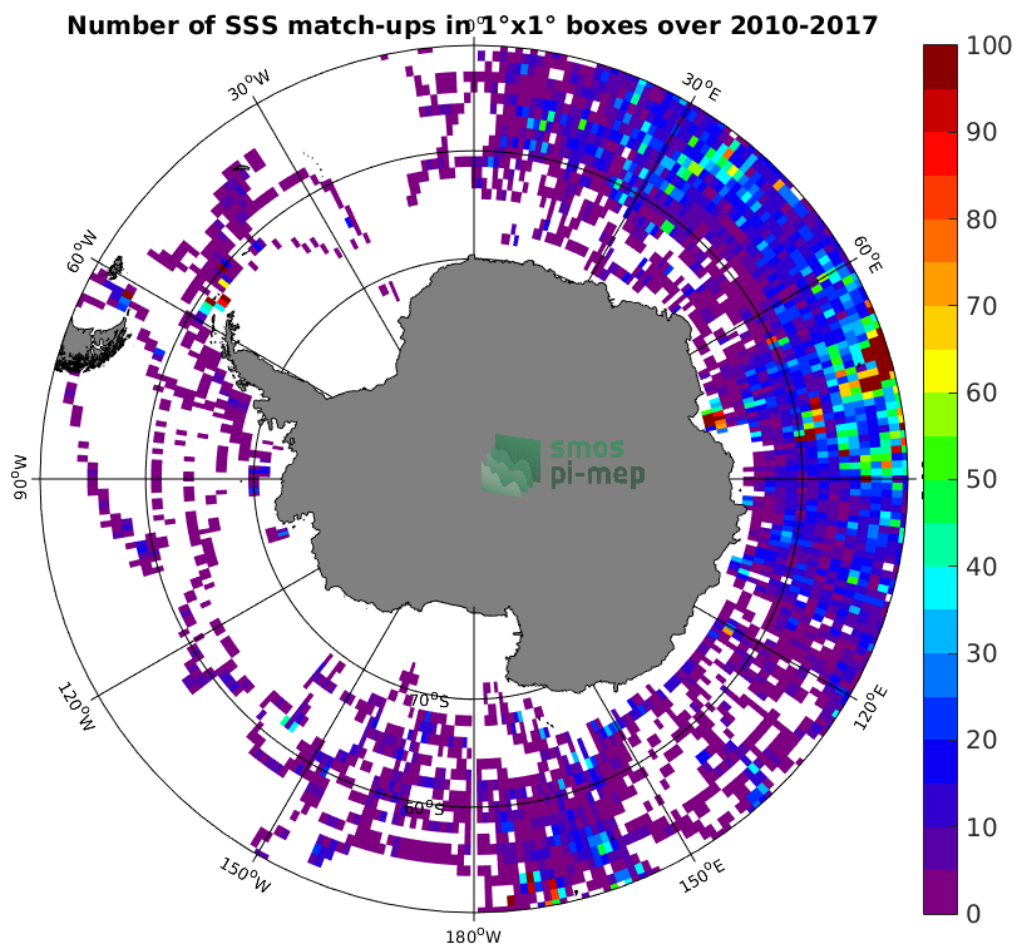
Figure 4: Number of SSS match-ups between Sea mammals SSS and the SMOS SSS L3 v317 - Monthly - 25 km (CATDS-CPDC) SSS product for the Southern Ocean Pi-MEP region over 1^\circ \times 1^\circ boxes and for the full satellite product period.
