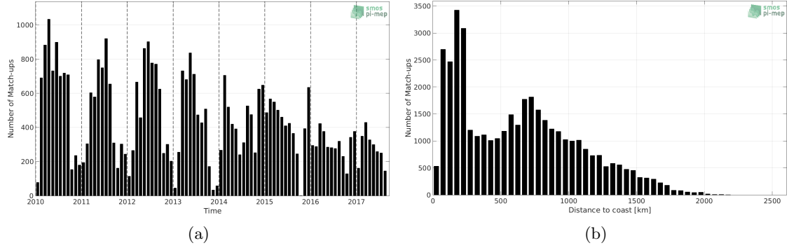
Figure 1: Number of match-ups between Sea mammals and SMOS-L3-CATDS-CPDC-V317-MONTHLY-25KM SSS as a function of time (a) and as function of the distance to coast (b) over the Southern Ocean Pi-MEP region and for the full satellite product period.
