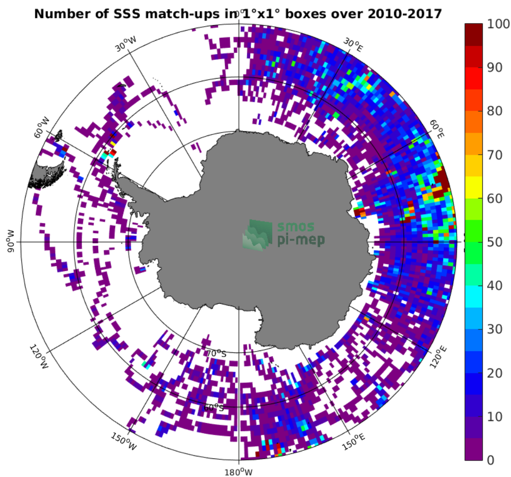
Figure 4: Number of SSS match-ups between Sea mammals SSS and the SMOS-L3-CATDS-CPDC-V317-MONTHLY-25KM SSS product for the Southern Ocean Pi-MEP region over 1^\circ \times 1^\circ boxes and for the full satellite product period.
