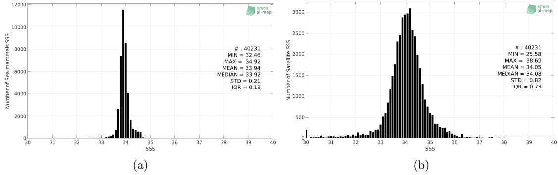
Figure 2: Histograms of SSS from Sea mammals (a) and SMOS-L3-CATDS-CPDC-V317-MONTHLY-25KM (b) considering all match-up pairs per bins of 0.1 over the Southern Ocean Pi-MEP region and for the full satellite product period.
