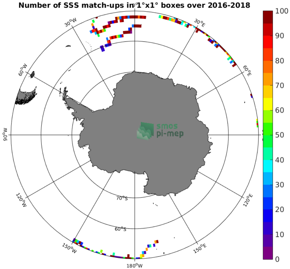
Figure 3: Number of SSS match-ups between Surface drifters SSS and the SMOS SSS L3 v317 - Monthly - 25 km (CATDS-CPDC) SSS product for the Southern Ocean Pi-MEP region over 1°x1° boxes and for the full satellite product period.
