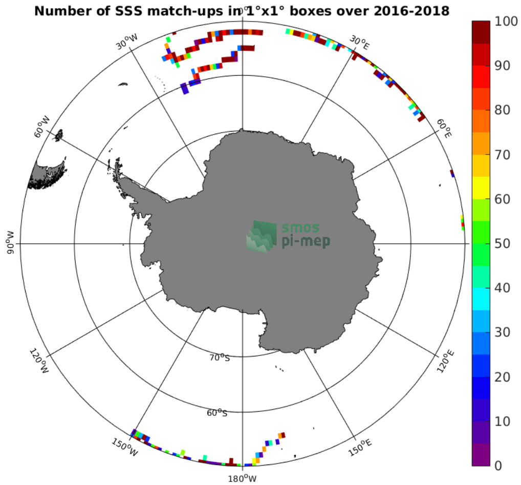
Figure 3: Number of SSS match-ups between Surface drifters SSS and the SMOS L3 v317 - Monthly - 25 km (CATDS-CPDC) SSS product for the Southern Ocean Pi-MEP region over 1°x1° boxes and for the full satellite product period.
