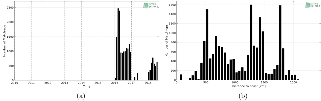
Figure 1: Number of match-ups between Surface drifters and SMOS L3 v317 - Monthly - 25 km (CATDS-CPDC) SSS as a function of time (a) and as function of the distance to coast (b) over the Southern Ocean Pi-MEP region and for the full satellite product period.
