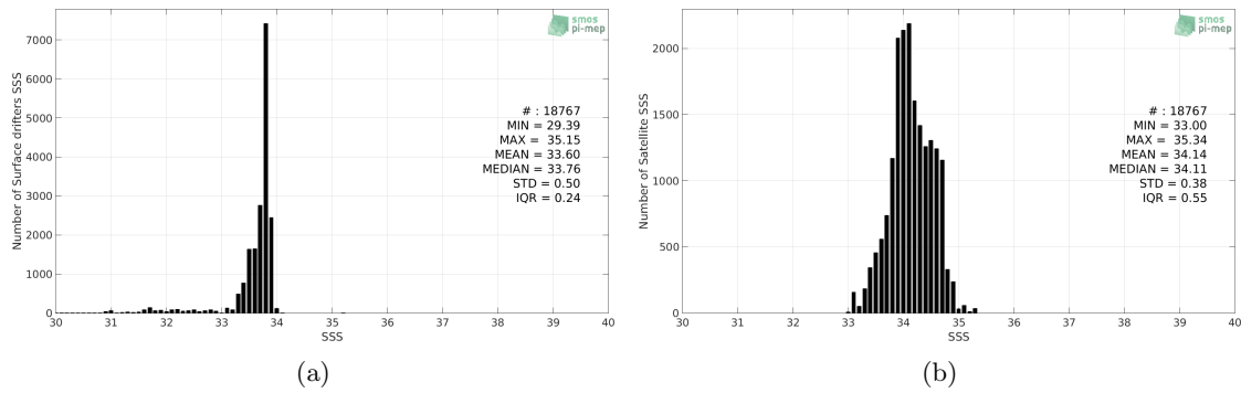
Figure 2: Histograms of SSS from Surface drifters (a) and SMOS L3 v317 - Monthly - 25 km (CATDS-CPDC) (b) considering all match-up pairs per bins of 0.1 over the Southern Ocean Pi-MEP region and for the full satellite product period.
