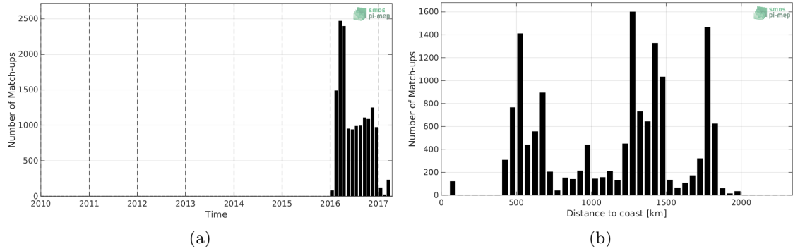
Figure 1: Number of match-ups between Surface drifters and SMOS-L3-CATDS-CPDC-V317-MONTHLY-25KM SSS as a function of time (a) and as function of the distance to coast (b) over the Southern Ocean Pi-MEP region and for the full satellite product period.
