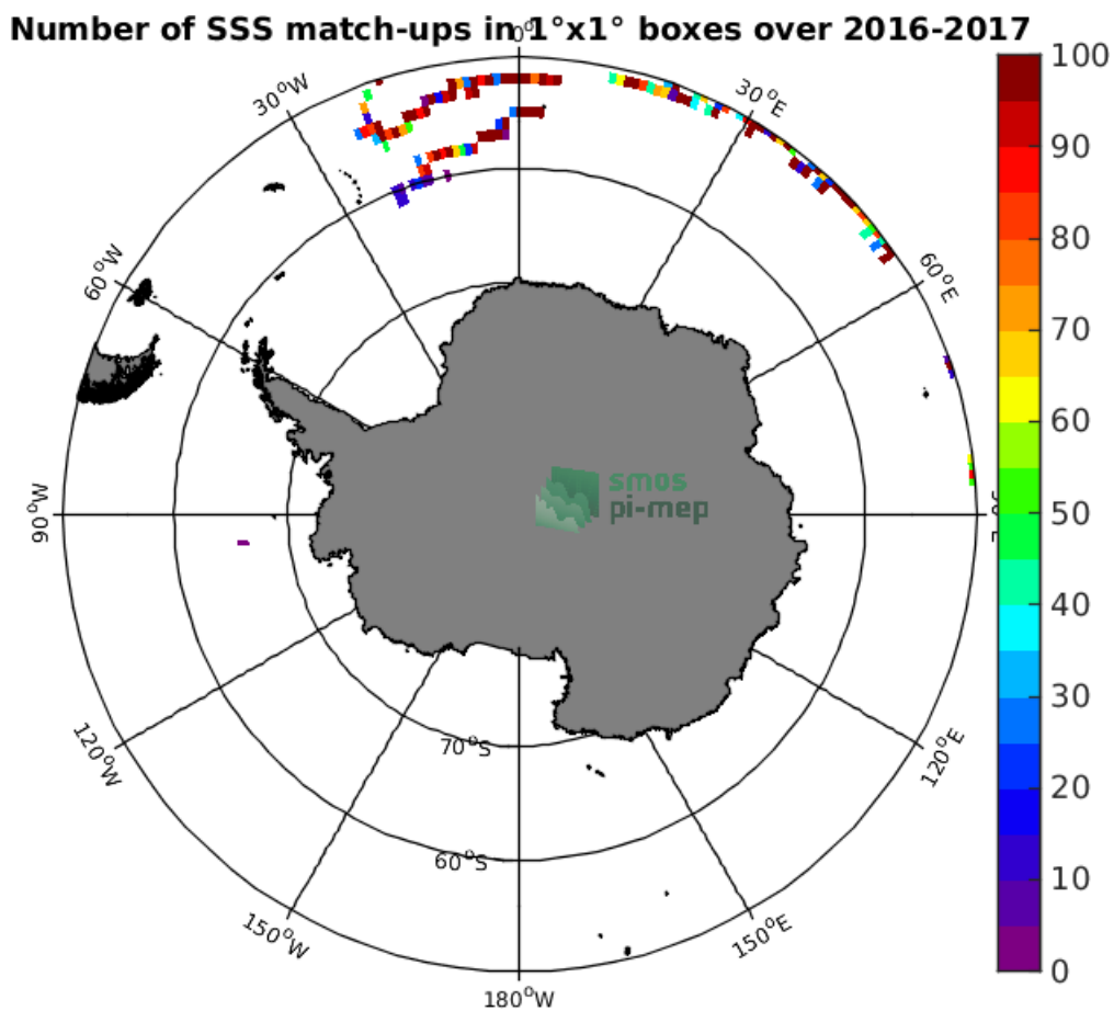
Figure 3: Number of SSS match-ups between Surface drifters SSS and the SMOS-L3-CATDS-CPDC-V317-MONTHLY-25KM SSS product for the Southern Ocean Pi-MEP region over 1^\circ \times 1^\circ boxes and for the full satellite product period.
