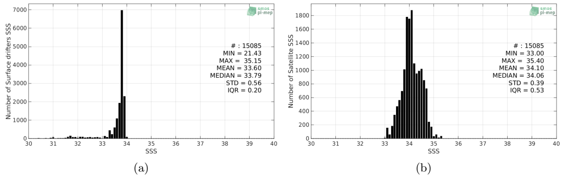
Figure 2: Histograms of SSS from Surface drifters (a) and SMOS-L3-CATDS-CPDC-V317-MONTHLY-25KM (b) considering all match-up pairs per bins of 0.1 over the Southern Ocean Pi-MEP region and for the full satellite product period.
