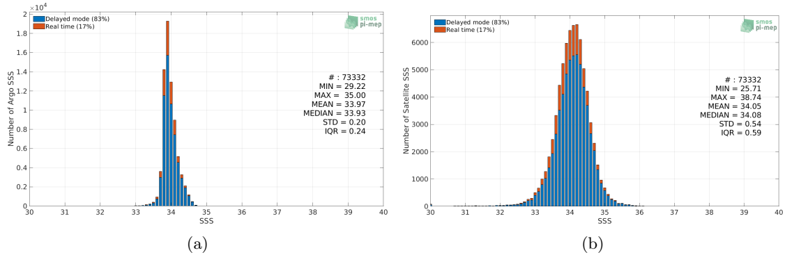
Figure 2: Histograms of SSS from Argo (a) and SMOS SSS L3 v317 - Monthly - 25 km (CATDS-CPDC) (b) considering all match-up pairs per bins of 0.1 over the Southern Ocean Pi-MEP region and for the full satellite product period.
