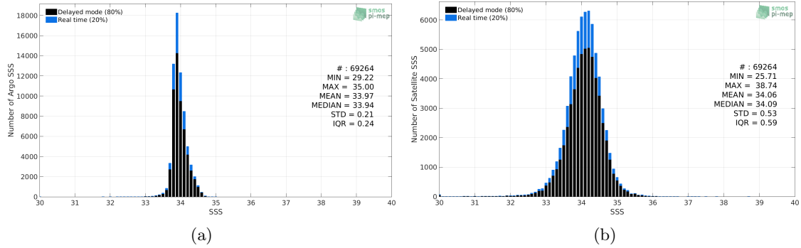
Figure 2: Histograms of SSS from Argo (a) and SMOS SSS L3 v317 - Monthly - 25 km (CATDS-CPDC) (b) considering all match-up pairs per bins of 0.1 over the Southern Ocean Pi-MEP region and for the full satellite product period.
