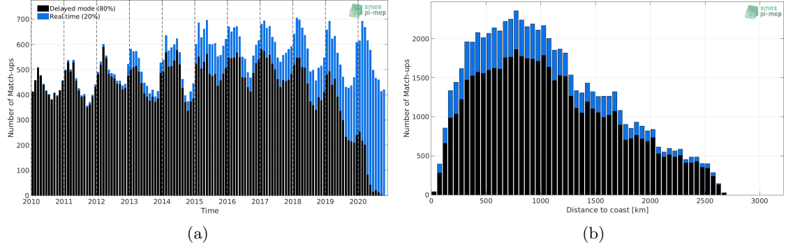
Figure 1: Number of match-ups between Argo and SMOS SSS L3 v317 - Monthly - 25 km (CATDS-CPDC) SSS as a function of time (a) and as function of the distance to coast (b) over the Southern Ocean Pi-MEP region and for the full satellite product period.
