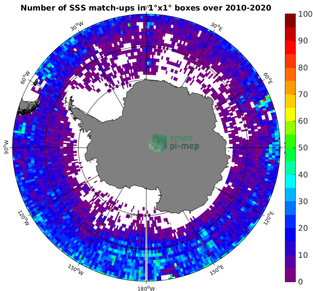
Figure 4: Number of SSS match-ups between Argo SSS and the SMOS SSS L3 v317 - Monthly - 25 km (CATDS-CPDC) SSS product for the Southern Ocean Pi-MEP region over 1^\circ \times 1^\circ boxes and for the full satellite product period.
