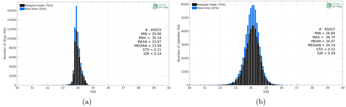
Figure 2: Histograms of SSS from Argo (a) and SMOS L3 v317 - Monthly - 25 km (CATDS-CPDC) (b) considering all match-up pairs per bins of 0.1 over the Southern Ocean Pi-MEP region and for the full satellite product period.
