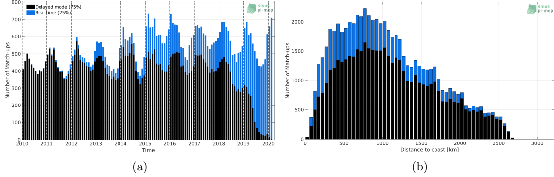
Figure 1: Number of match-ups between Argo and SMOS L3 v317 - Monthly - 25 km (CATDS-CPDC) SSS as a function of time (a) and as function of the distance to coast (b) over the Southern Ocean Pi-MEP region and for the full satellite product period.
