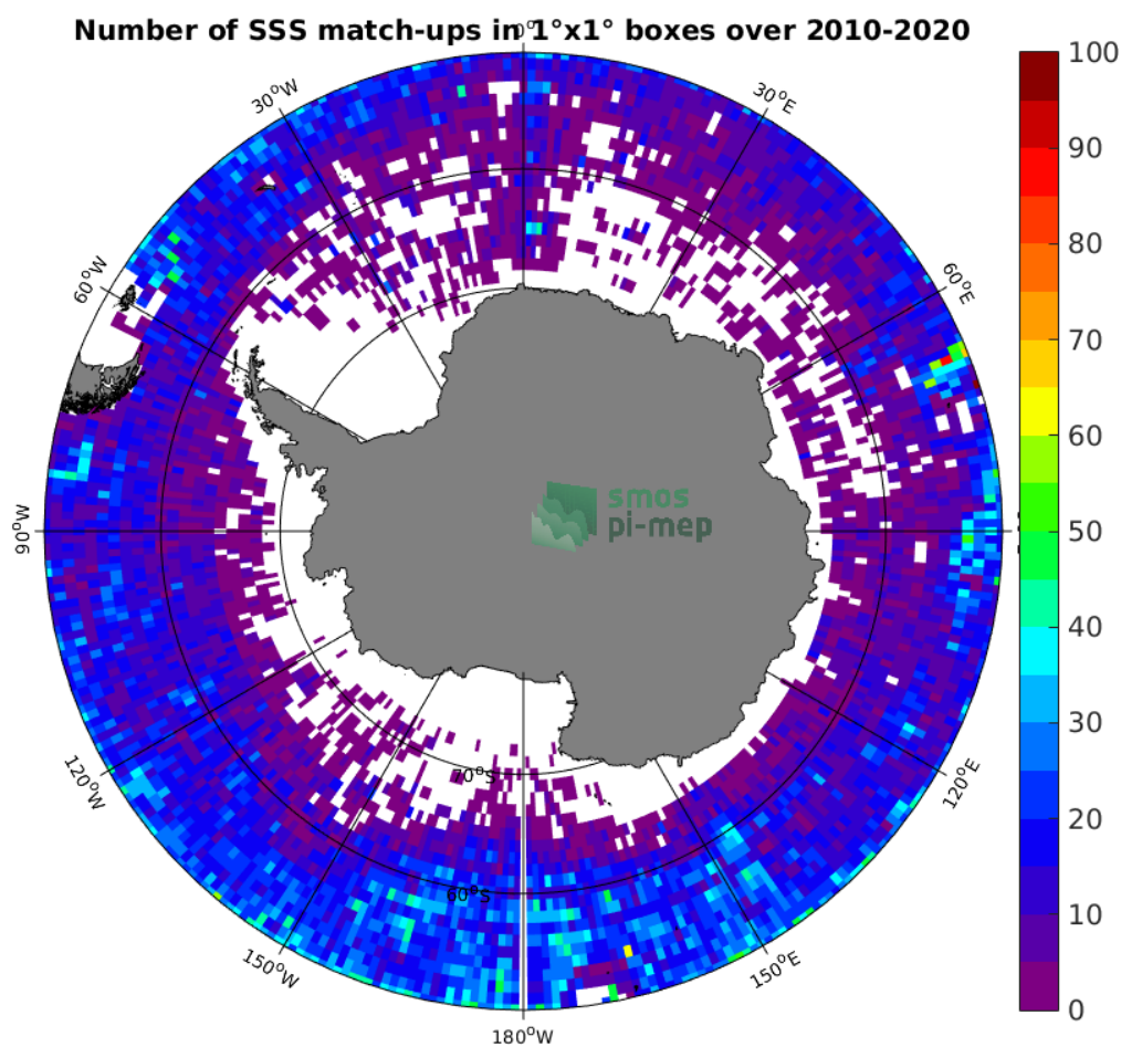
Figure 4: Number of SSS match-ups between Argo SSS and the SMOS L3 v317 - Monthly - 25 km (CATDS-CPDC) SSS product for the Southern Ocean Pi-MEP region over 1^\circ \times 1^\circ boxes and for the full satellite product period.
