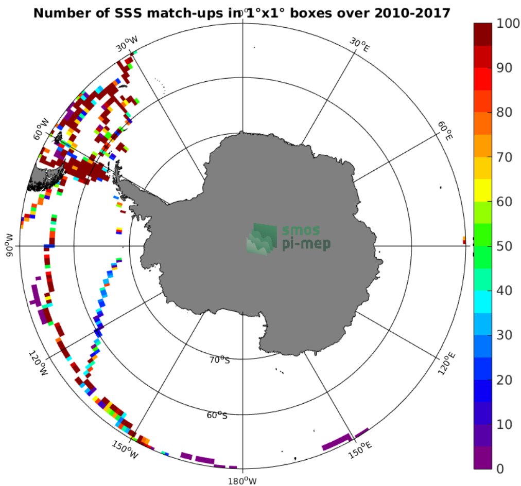
Figure 4: Number of SSS match-ups between TSG-GOSUD-Sailing-ship SSS and the SMOS L3 v317 - 10 Days - 25 km (CATDS-CPDC) SSS product for the Southern Ocean Pi-MEP region over 1°x1° boxes and for the full satellite product period.
