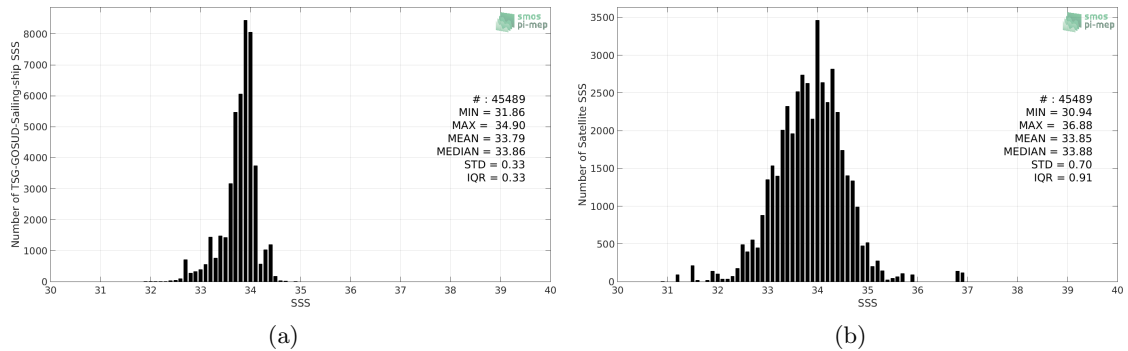
Figure 2: Histograms of SSS from TSG-GOSUD-Sailing-ship (a) and SMOS L3 v317 - 10 Days - 25 km (CATDS-CPDC) (b) considering all match-up pairs per bins of 0.1 over the Southern Ocean Pi-MEP region and for the full satellite product period.
