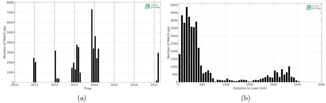
Figure 1: Number of match-ups between TSG-GOSUD-Sailing-ship and SMOS L3 v317 - 10 Days - 25 km (CATDS-CPDC) SSS as a function of time (a) and as function of the distance to coast (b) over the Southern Ocean Pi-MEP region and for the full satellite product period.
