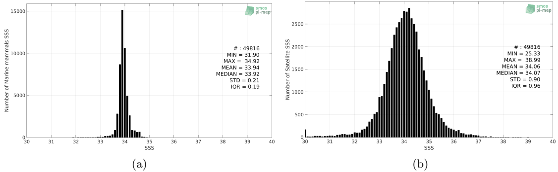
Figure 2: Histograms of SSS from Marine mammals (a) and SMOS SSS L3 v317 - 10 Days - 25 km (CATDS-CPDC) (b) considering all match-up pairs per bins of 0.1 over the Southern Ocean Pi-MEP region and for the full satellite product period.
