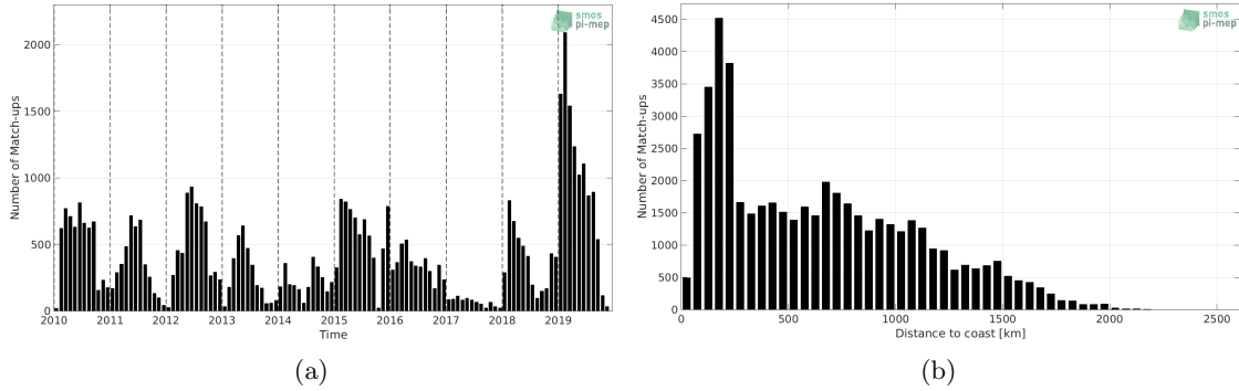
Figure 1: Number of match-ups between Marine mammals and SMOS SSS L3 v317 - 10 Days - 25 km (CATDS-CPDC) SSS as a function of time (a) and as function of the distance to coast (b) over the Southern Ocean Pi-MEP region and for the full satellite product period.
