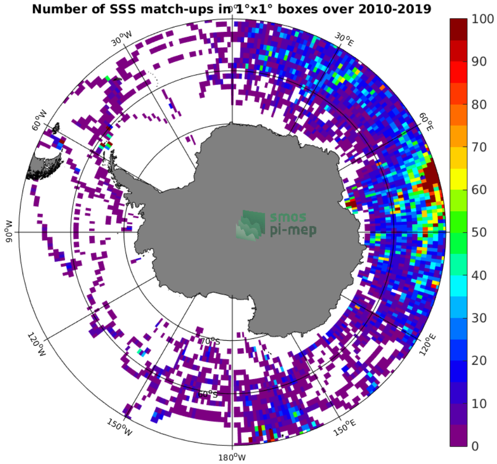
Figure 4: Number of SSS match-ups between Marine mammals SSS and the SMOS SSS L3 v317 - 10 Days - 25 km (CATDS-CPDC) SSS product for the Southern Ocean Pi-MEP region over 1^\circ \times 1^\circ boxes and for the full satellite product period.
