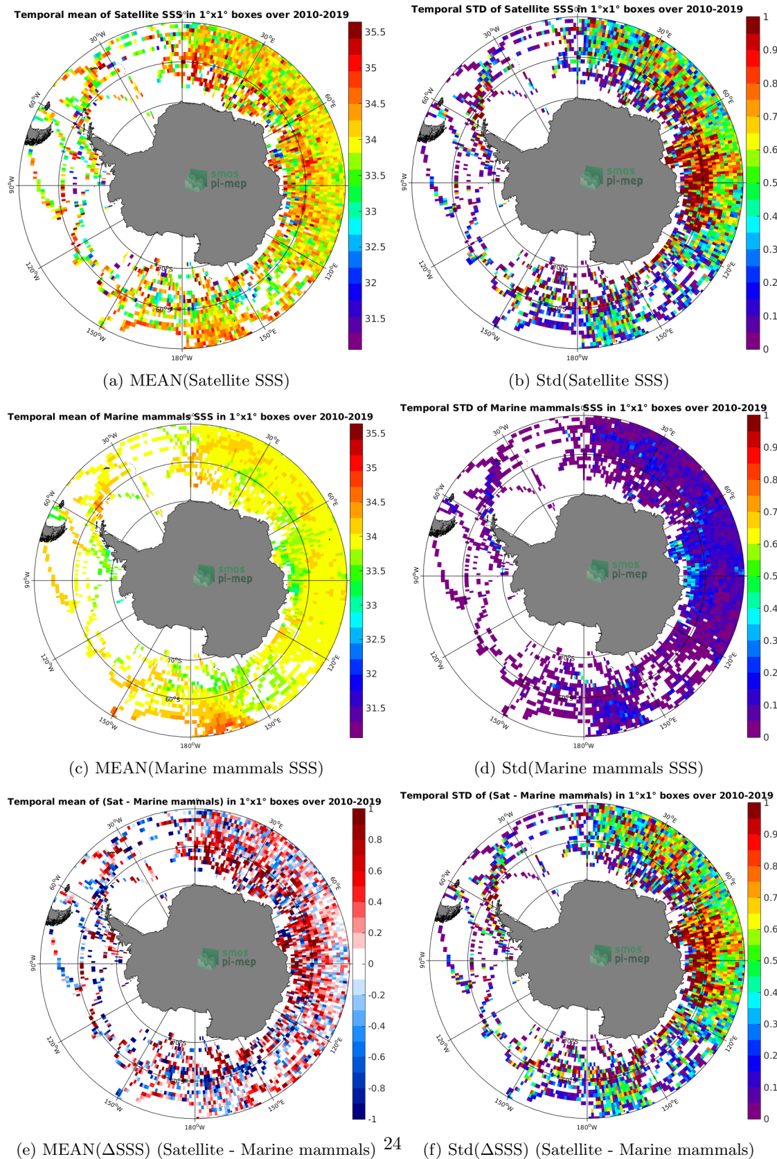
Figure 6: Temporal mean (left) and Std (right) of SSS from SMOS SSS L3 v317 - 10 Days - 25 km (CATDS-CPDC) (top), Marine mammals (middle), and of \Delta SSS (Satellite - Marine mammals). Only match-up pairs are used to generate these maps.
