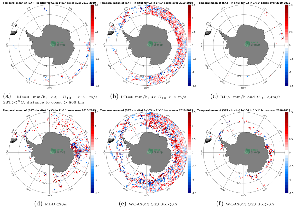
Figure 12: Temporal mean gridded over spatial boxes of size 1^{\circ} \times 1^{\circ} of \Delta\text{SSS} (SMOS SSS L3 v317 - 10 Days - 25 km (CATDS-CPDC) - Marine mammals) for 6 different subdatasets corresponding to: RR=0 mm/h, 3 < U_{10} < 12 m/s, SST > 5^{\circ}\text{C} , distance to coast > 800 km (a), RR=0 mm/h, 3 < U_{10} < 12 m/s (b), RR > 1 mm/h and U_{10} < 4 m/s (c), MLD < 20\text{m} (d), WOA2013 SSS Std < 0.2 (e), WOA2013 SSS Std > 0.2 (f).
