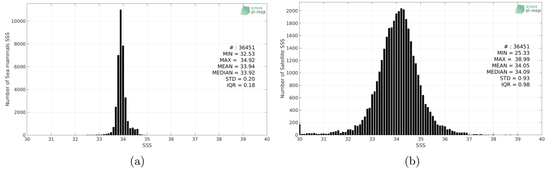
Figure 2: Histograms of SSS from Sea mammals (a) and SMOS SSS L3 v317 - 10 Days - 25 km (CATDS-CPDC) (b) considering all match-up pairs per bins of 0.1 over the Southern Ocean Pi-MEP region and for the full satellite product period.
