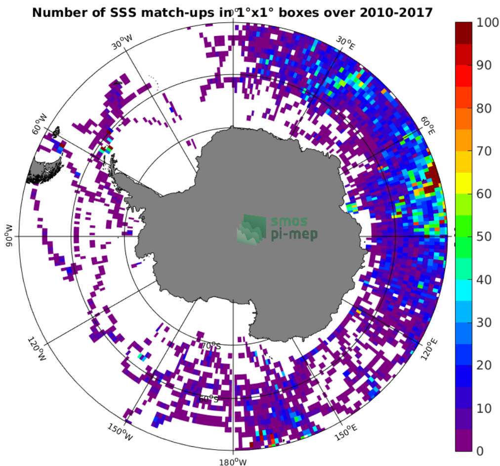
Figure 4: Number of SSS match-ups between Sea mammals SSS and the SMOS SSS L3 v317 - 10 Days - 25 km (CATDS-CPDC) SSS product for the Southern Ocean Pi-MEP region over 1^\circ \times 1^\circ boxes and for the full satellite product period.
