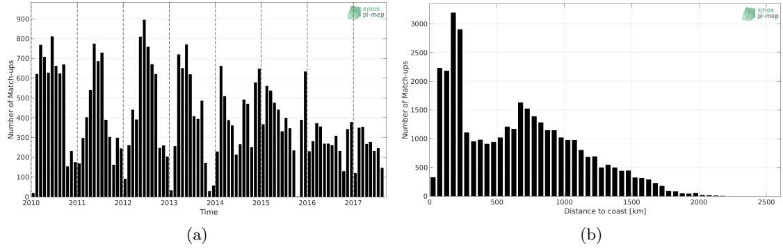
Figure 1: Number of match-ups between Sea mammals and SMOS SSS L3 v317 - 10 Days - 25 km (CATDS-CPDC) SSS as a function of time (a) and as function of the distance to coast (b) over the Southern Ocean Pi-MEP region and for the full satellite product period.
