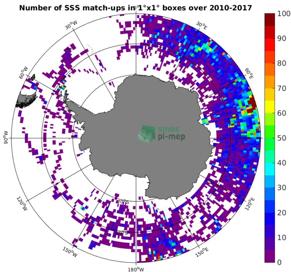
Figure 4: Number of SSS match-ups between Sea mammals SSS and the SMOS L3 v317 - 10 Days - 25 km (CATDS-CPDC) SSS product for the Southern Ocean Pi-MEP region over 1^\circ \times 1^\circ boxes and for the full satellite product period.
