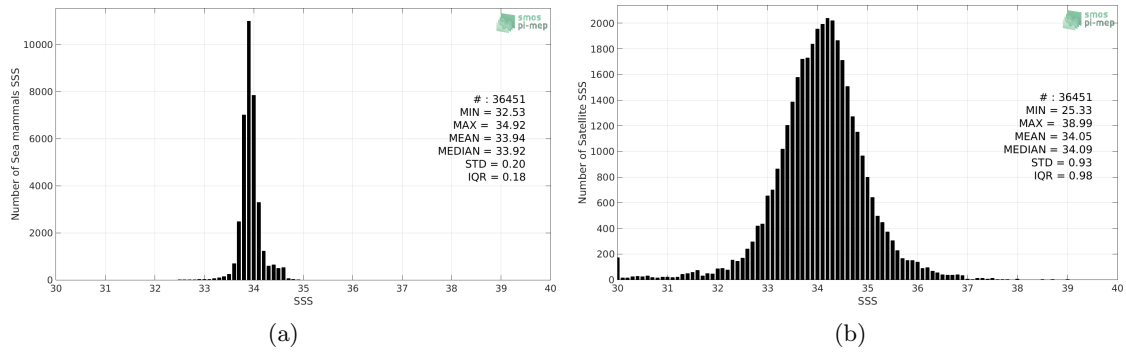
Figure 2: Histograms of SSS from Sea mammals (a) and SMOS L3 v317 - 10 Days - 25 km (CATDS-CPDC) (b) considering all match-up pairs per bins of 0.1 over the Southern Ocean Pi-MEP region and for the full satellite product period.
