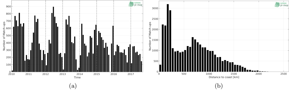
Figure 1: Number of match-ups between Sea mammals and SMOS L3 v317 - 10 Days - 25 km (CATDS-CPDC) SSS as a function of time (a) and as function of the distance to coast (b) over the Southern Ocean Pi-MEP region and for the full satellite product period.
