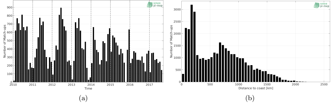
Figure 1: Number of match-ups between Sea mammals and SMOS-L3-CATDS-CPDC-V317-10DAYS-25KM SSS as a function of time (a) and as function of the distance to coast (b) over the Southern Ocean Pi-MEP region and for the full satellite product period.
