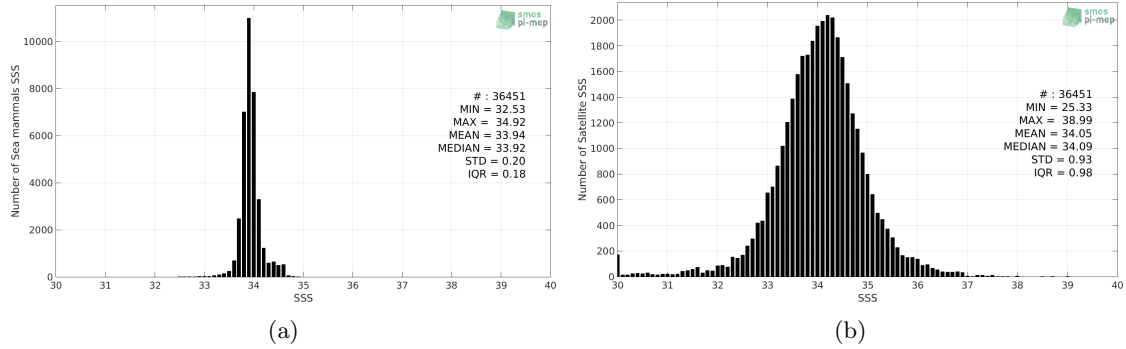
Figure 2: Histograms of SSS from Sea mammals (a) and SMOS-L3-CATDS-CPDC-V317-10DAYS-25KM (b) considering all match-up pairs per bins of 0.1 over the Southern Ocean Pi-MEP region and for the full satellite product period.
