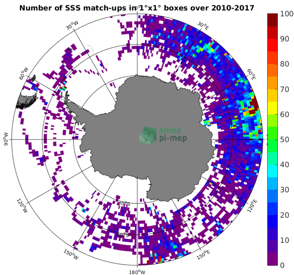
Figure 4: Number of SSS match-ups between Sea mammals SSS and the SMOS-L3-CATDS-CPDC-V317-10DAYS-25KM SSS product for the Southern Ocean Pi-MEP region over 1^\circ \times 1^\circ boxes and for the full satellite product period.
