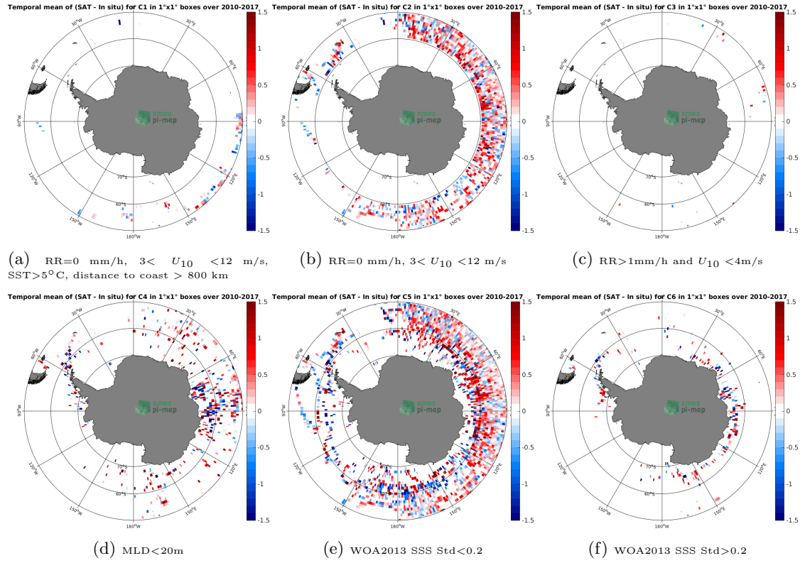
Figure 12: Temporal mean gridded over spatial boxes of size 1^\circ \times 1^\circ of \Delta SSS (SMOS-L3-CATDS-CPDC-V317-10DAYS-25KM - Sea mammals) for 6 different subdatasets corresponding to: RR=0 mm/h, 3 < U_{10} < 12 m/s, SST >5^\circ C, distance to coast > 800 km (a), RR=0 mm/h, 3 < U_{10} < 12 m/s (b), RR >1 mm/h and U_{10} < 4 m/s (c), MLD <20 m (d), WOA2013 SSS Std <0.2 (e), WOA2013 SSS Std >0.2 (f).
