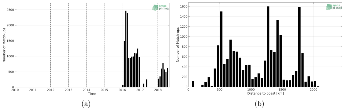
Figure 1: Number of match-ups between Surface drifters and SMOS SSS L3 v317 - 10 Days - 25 km (CATDS-CPDC) SSS as a function of time (a) and as function of the distance to coast (b) over the Southern Ocean Pi-MEP region and for the full satellite product period.
