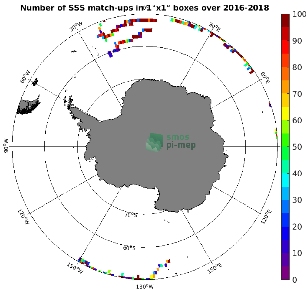
Figure 3: Number of SSS match-ups between Surface drifters SSS and the SMOS SSS L3 v317 - 10 Days - 25 km (CATDS-CPDC) SSS product for the Southern Ocean Pi-MEP region over 1^\circ \times 1^\circ boxes and for the full satellite product period.
