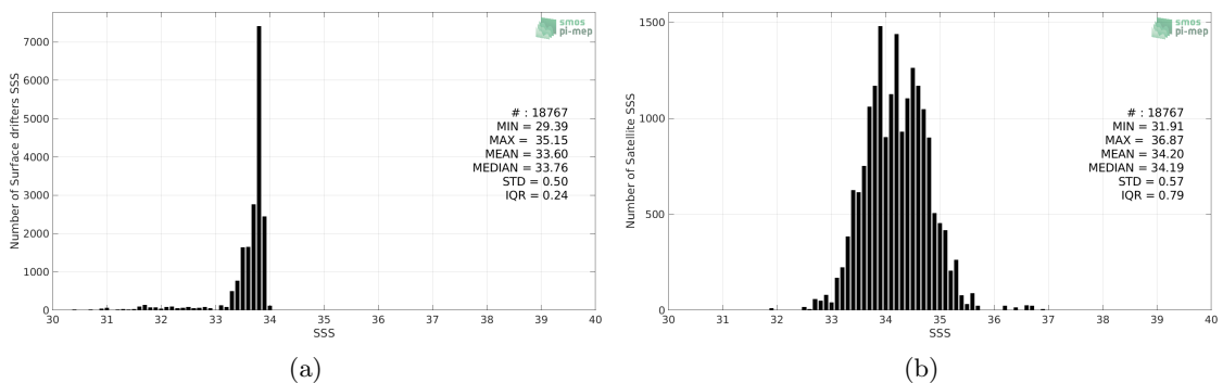
Figure 2: Histograms of SSS from Surface drifters (a) and SMOS SSS L3 v317 - 10 Days - 25 km (CATDS-CPDC) (b) considering all match-up pairs per bins of 0.1 over the Southern Ocean Pi-MEP region and for the full satellite product period.
