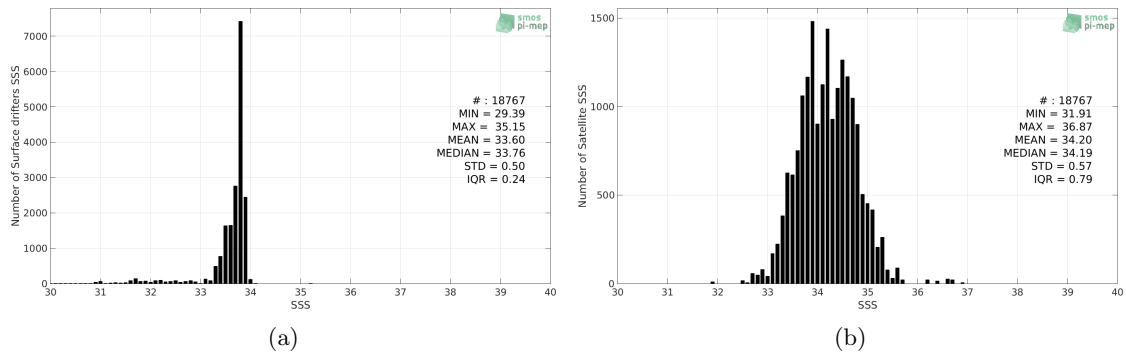
Figure 2: Histograms of SSS from Surface drifters (a) and SMOS L3 v317 - 10 Days - 25 km (CATDS-CPDC) (b) considering all match-up pairs per bins of 0.1 over the Southern Ocean Pi-MEP region and for the full satellite product period.
