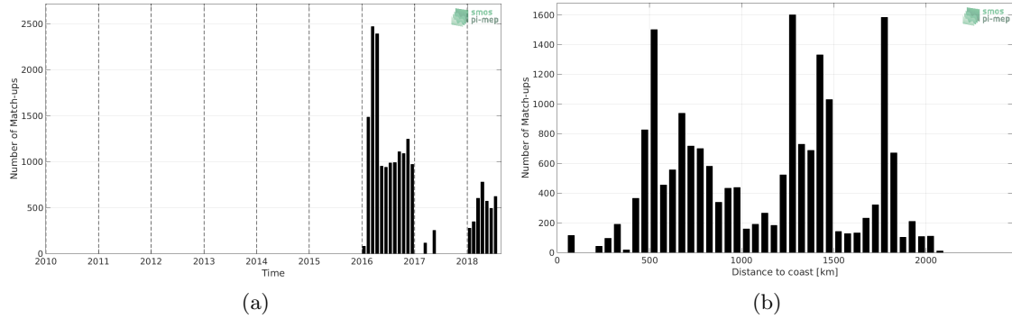
Figure 1: Number of match-ups between Surface drifters and SMOS L3 v317 - 10 Days - 25 km (CATDS-CPDC) SSS as a function of time (a) and as function of the distance to coast (b) over the Southern Ocean Pi-MEP region and for the full satellite product period.
