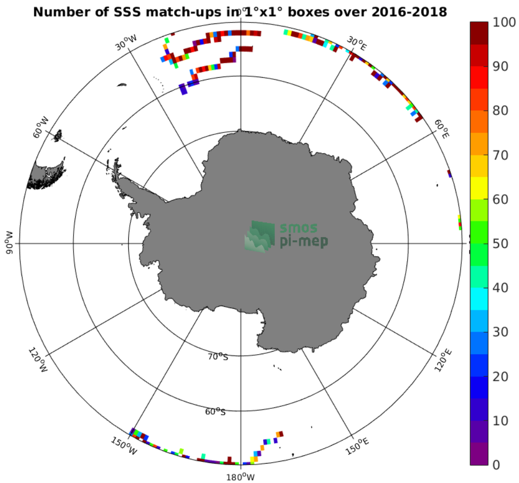
Figure 3: Number of SSS match-ups between Surface drifters SSS and the SMOS L3 v317 - 10 Days - 25 km (CATDS-CPDC) SSS product for the Southern Ocean Pi-MEP region over 1^{\circ} \times 1^{\circ} boxes and for the full satellite product period.
