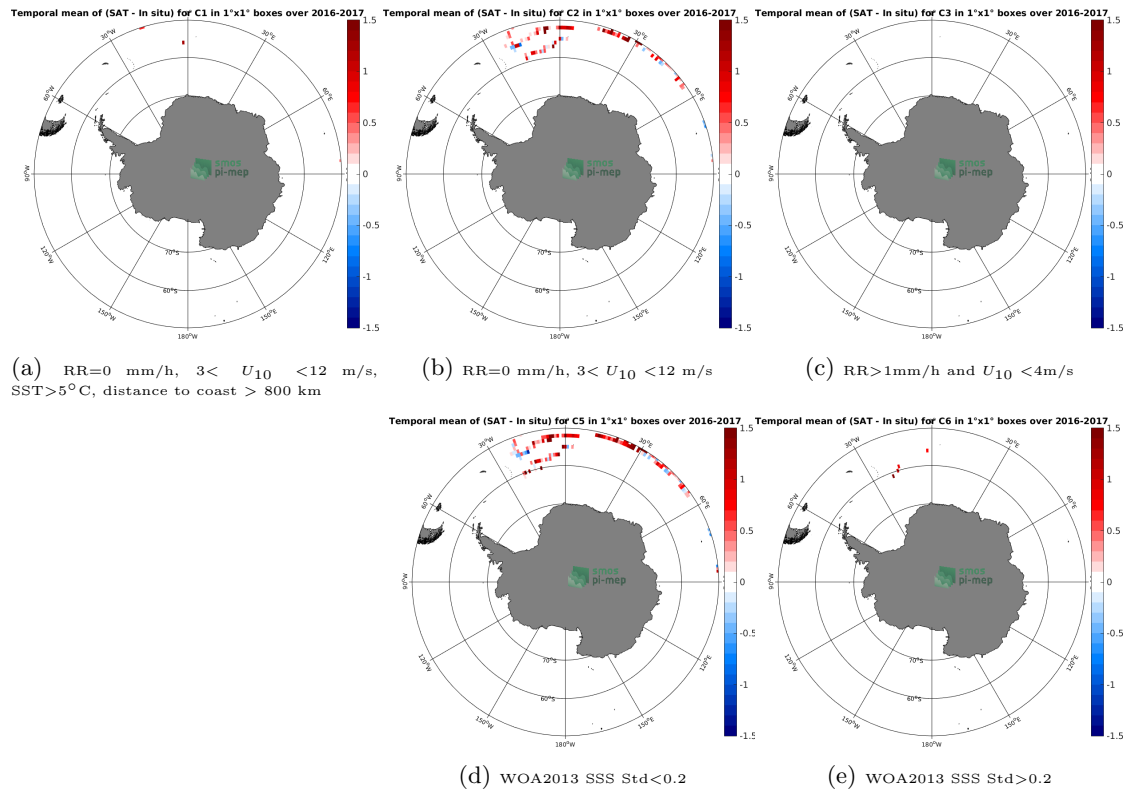
Figure 11: Temporal mean gridded over spatial boxes of size 1^\circ \times 1^\circ of \Delta SSS (SMOS-L3-CATDS-CPDC-V317-10DAYS-25KM - Surface drifters) for 5 different subdatasets corresponding to:RR=0 mm/h, 3 < U_{10} < 12 m/s, SST >5^\circ C, distance to coast > 800 km (a), RR=0 mm/h, 3 < U_{10} < 12 m/s (b), RR >1 mm/h and U_{10} < 4 m/s (c), WOA2013 SSS Std <0.2 (d), WOA2013 SSS Std >0.2 (e).
