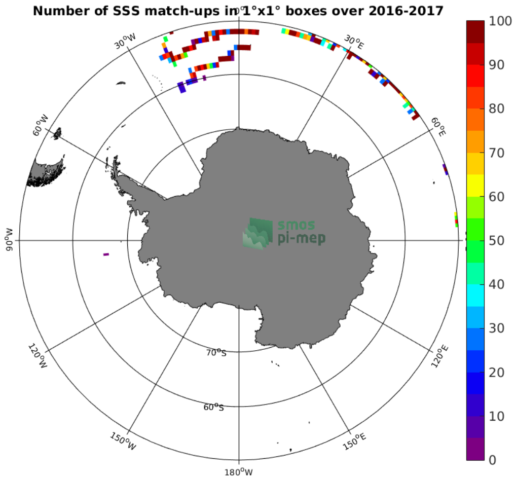
Figure 3: Number of SSS match-ups between Surface drifters SSS and the SMOS-L3-CATDS-CPDC-V317-10DAYS-25KM SSS product for the Southern Ocean Pi-MEP region over 1^\circ \times 1^\circ boxes and for the full satellite product period.
