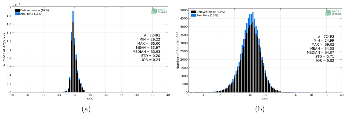
Figure 2: Histograms of SSS from Argo (a) and SMOS SSS L3 v317 - 10 Days - 25 km (CATDS-CPDC) (b) considering all match-up pairs per bins of 0.1 over the Southern Ocean Pi-MEP region and for the full satellite product period.
