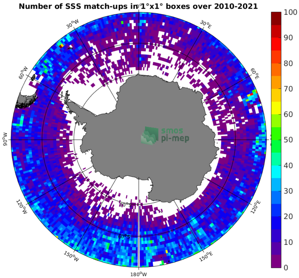
Figure 4: Number of SSS match-ups between Argo SSS and the SMOS SSS L3 v317 - 10 Days - 25 km (CATDS-CPDC) SSS product for the Southern Ocean Pi-MEP region over 1^\circ \times 1^\circ boxes and for the full satellite product period.
