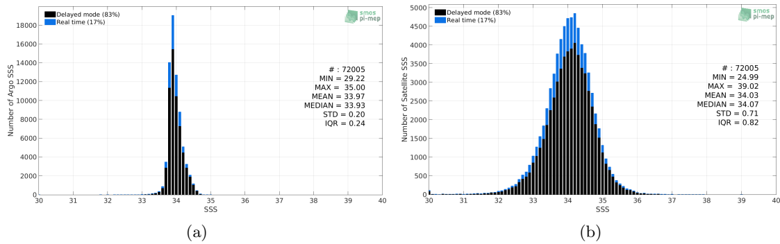
Figure 2: Histograms of SSS from Argo (a) and SMOS SSS L3 v317 - 10 Days - 25 km (CATDS-CPDC) (b) considering all match-up pairs per bins of 0.1 over the Southern Ocean Pi-MEP region and for the full satellite product period.
