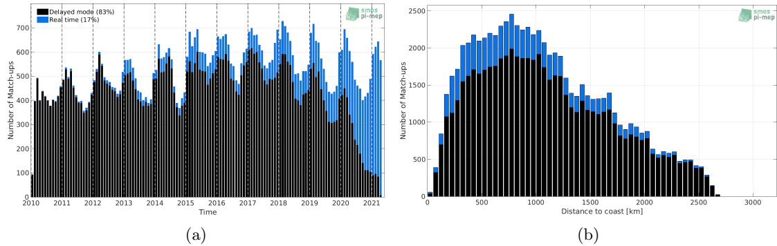
Figure 1: Number of match-ups between Argo and SMOS SSS L3 v317 - 10 Days - 25 km (CATDS-CPDC) SSS as a function of time (a) and as function of the distance to coast (b) over the Southern Ocean Pi-MEP region and for the full satellite product period.
