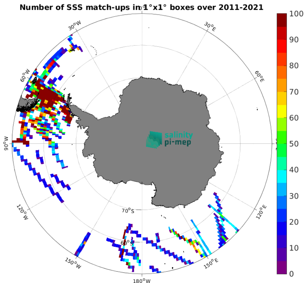
Figure 4: Number of SSS match-ups between TSG (SAMOS) SSS and the SMOS SSS L3 v2 - 9-Days (BEC) SSS product for the Southern Ocean Pi-MEP region over 1^\circ \times 1^\circ boxes and for the full satellite product period.
