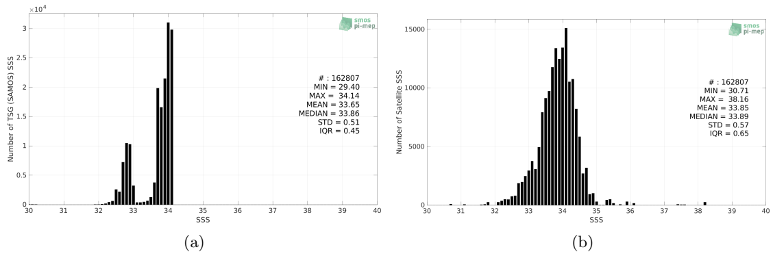
Figure 2: Histograms of SSS from TSG (SAMOS) (a) and SMOS SSS L3 v2 - 9-Days (BEC) (b) considering all match-up pairs per bins of 0.1 over the Southern Ocean Pi-MEP region and for the full satellite product period.
