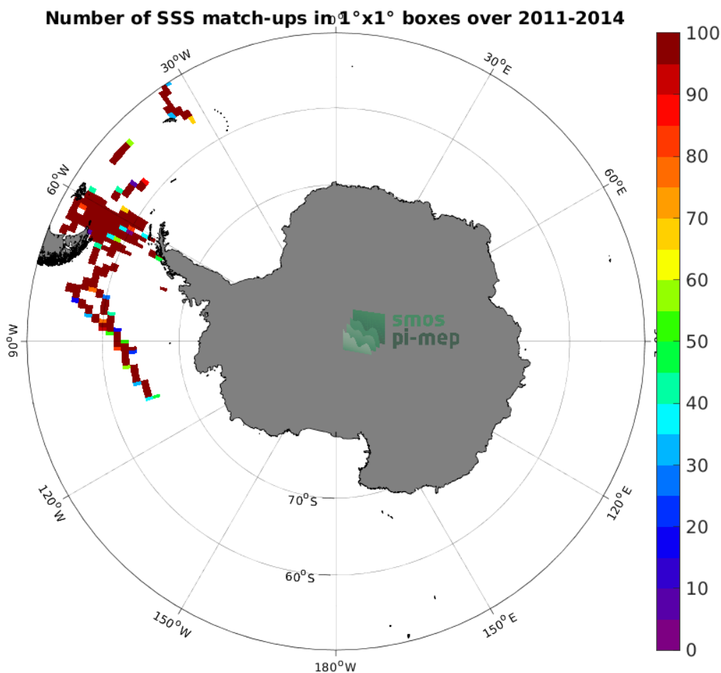
Figure 4: Number of SSS match-ups between TSG (SAMOS) SSS and the SMOS SSS L3 v2 - 9-Days (BEC) SSS product for the Southern Ocean Pi-MEP region over 1^{\circ} \times 1^{\circ} boxes and for the full satellite product period.
