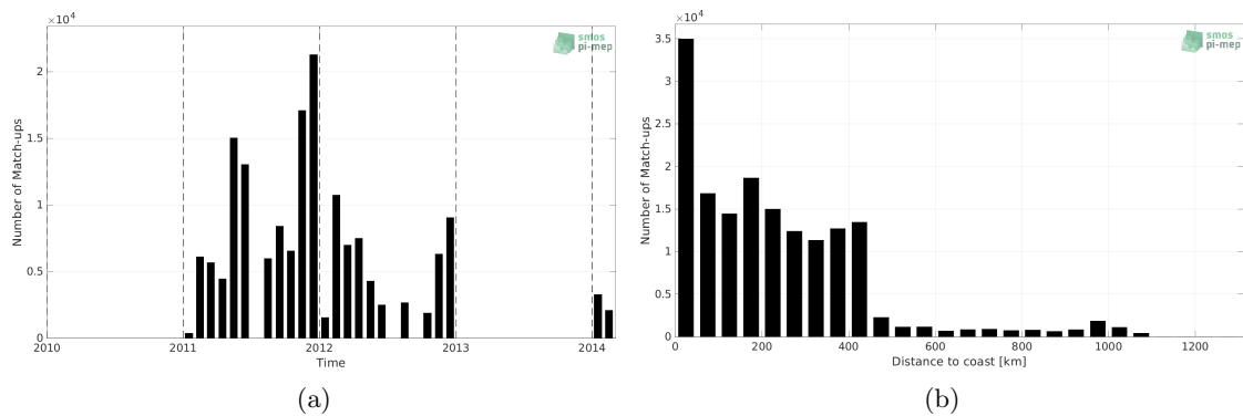
Figure 1: Number of match-ups between TSG (SAMOS) and SMOS SSS L3 v2 - 9-Days (BEC) SSS as a function of time (a) and as function of the distance to coast (b) over the Southern Ocean Pi-MEP region and for the full satellite product period.
