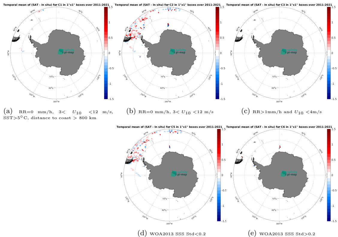
Figure 14: Temporal mean gridded over spatial boxes of size 1^\circ \times 1^\circ of \Delta\text{SSS} (SMOS SSS L3 v2 - 9-Days (BEC) - TSG (Polarstern)) for 5 different subdatasets corresponding to: RR=0 mm/h, 3 < U_{10} < 12 m/s, SST > 5^\circ\text{C} , distance to coast > 800 km (a), RR=0 mm/h, 3 < U_{10} < 12 m/s (b), RR > 1 mm/h and U_{10} < 4 m/s (c), WOA2013 SSS Std < 0.2 (d), WOA2013 SSS Std > 0.2 (e).
