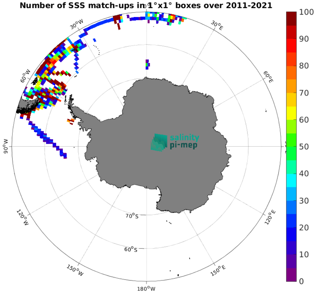
Figure 5: Number of SSS match-ups between TSG (Polarstern) SSS and the SMOS SSS L3 v2 - 9-Days (BEC) SSS product for the Southern Ocean Pi-MEP region over 1^\circ \times 1^\circ boxes and for the full satellite product period.
