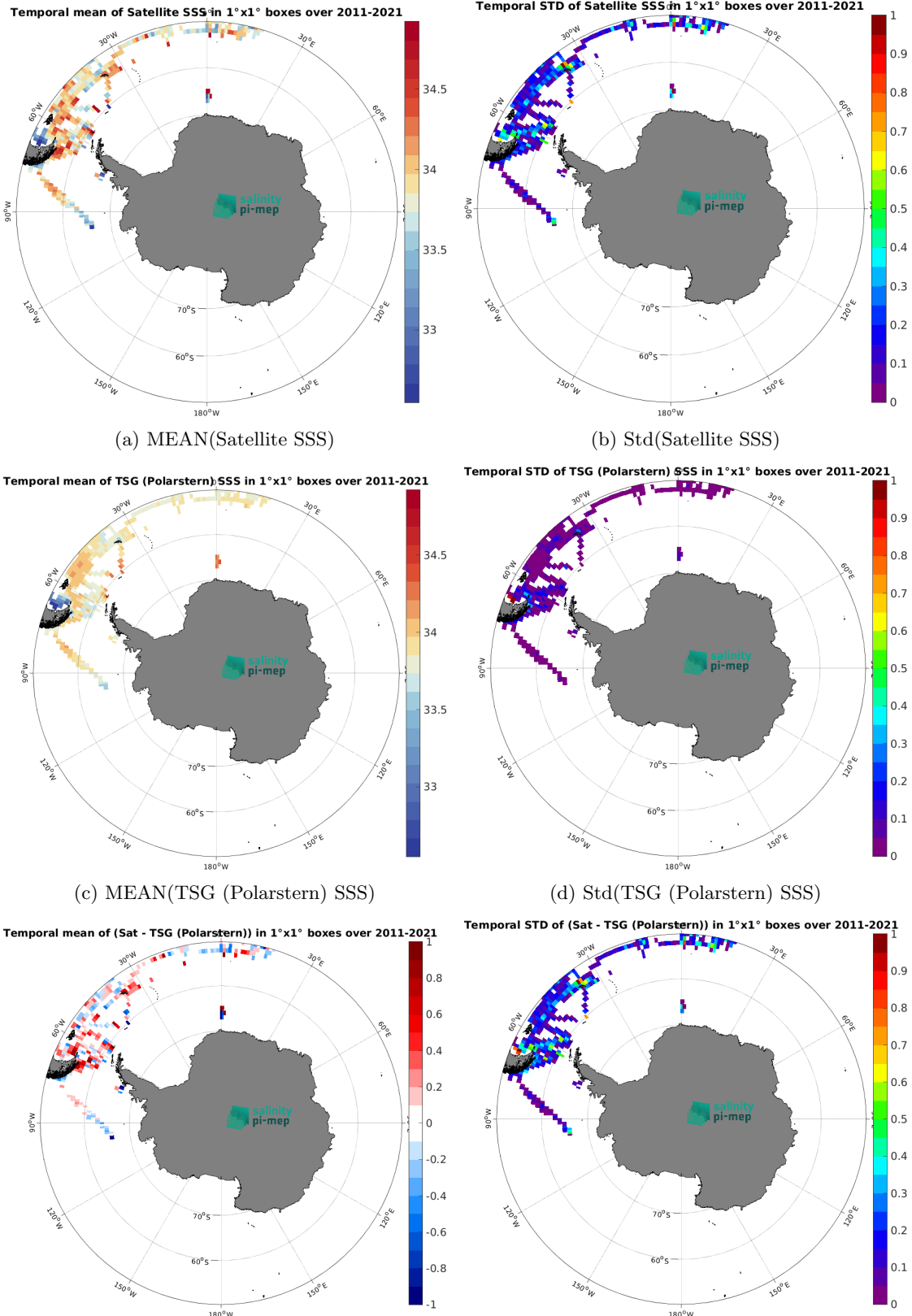
Figure 7: Temporal mean (left) and Std (right) of SSS from SMOS SSS L3 v2 - 9-Days (BEC) (top), TSG (Polarstern) (middle), and of \Delta SSS (Satellite - TSG (Polarstern)). Only match-up pairs are used to generate these maps.
