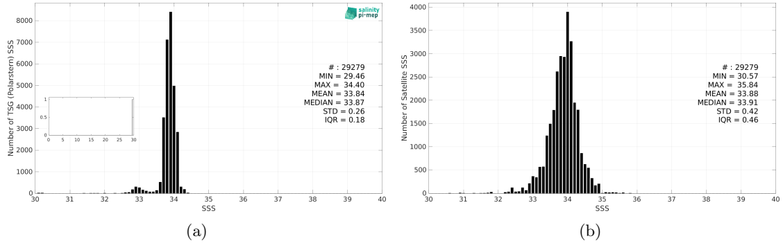
Figure 3: Histograms of SSS from TSG (Polarstern) (a) and SMOS SSS L3 v2 - 9-Days (BEC) (b) considering all match-up pairs per bins of 0.1 over the Southern Ocean Pi-MEP region and for the full satellite product period.
