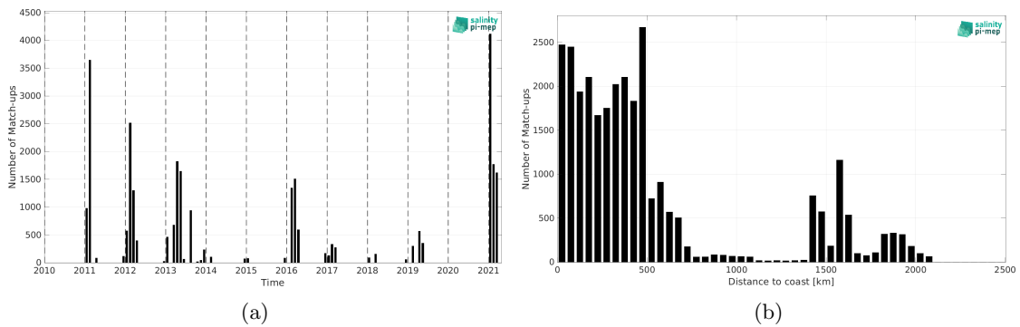
Figure 2: Number of match-ups between TSG (Polarstern) and SMOS SSS L3 v2 - 9-Days (BEC) SSS as a function of time (a) and as function of the distance to coast (b) over the Southern Ocean Pi-MEP region and for the full satellite product period.
