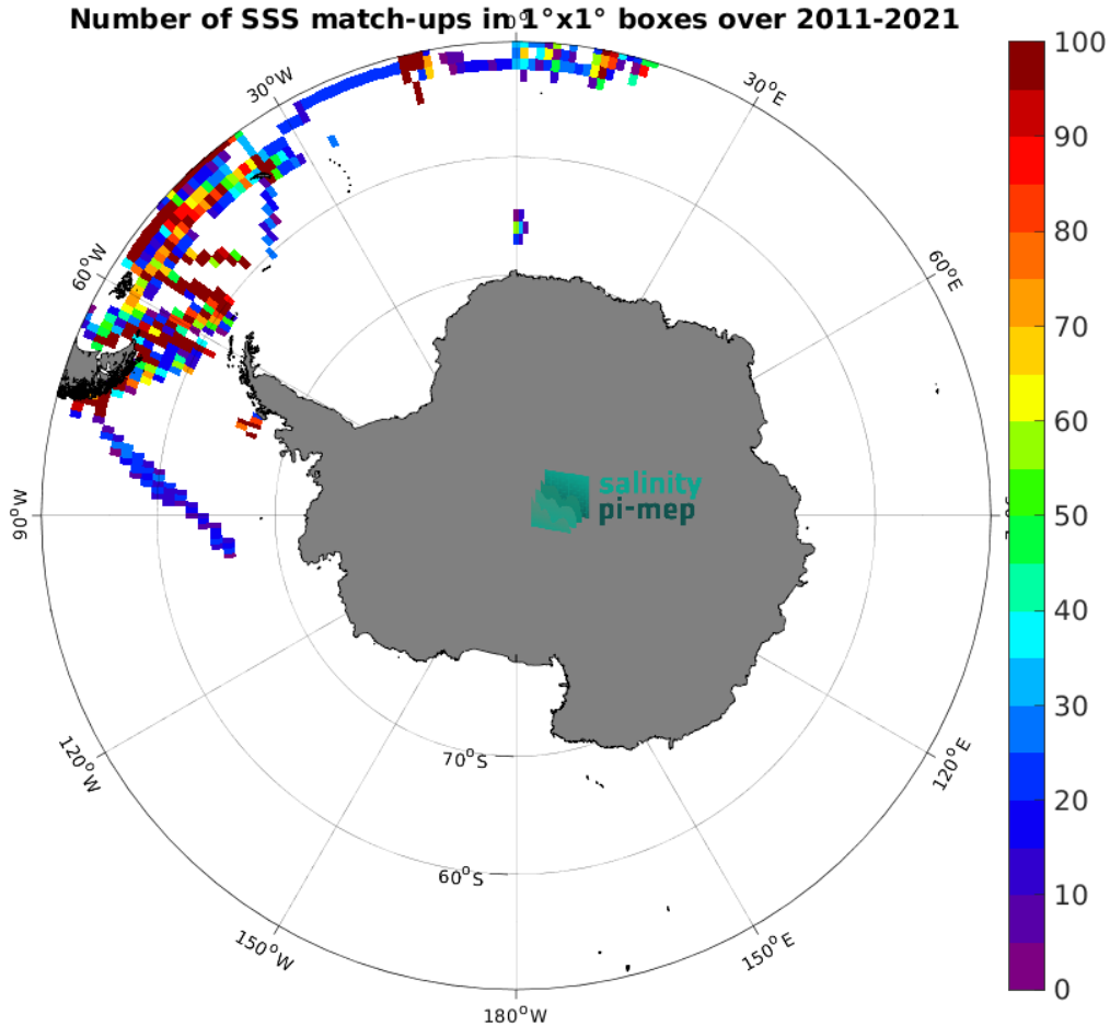
Figure 4: Number of SSS match-ups between TSG (Polarstern) SSS and the SMOS SSS L3 v2 - 9-Days (BEC) SSS product for the Southern Ocean Pi-MEP region over 1^\circ \times 1^\circ boxes and for the full satellite product period.
