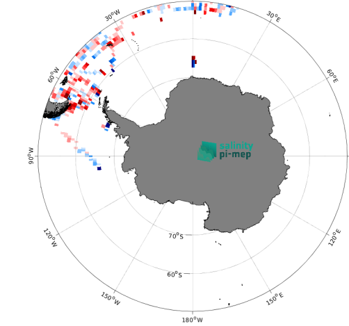
(e) MEAN( \Delta SSS) (Satellite - TSG (Polarstern)) 16
