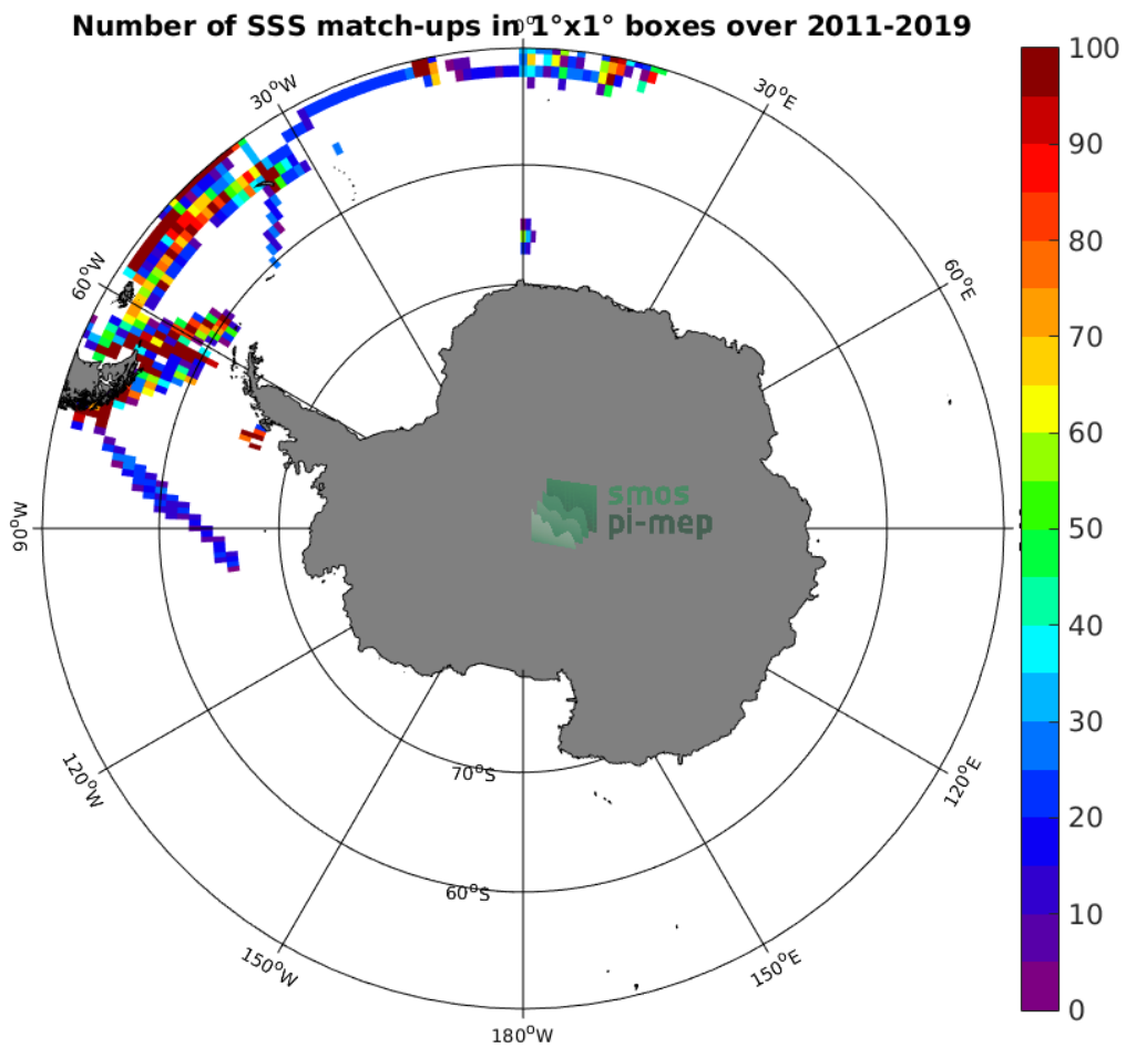
Figure 4: Number of SSS match-ups between TSG (Polarstern) SSS and the SMOS L3 v2 - 9-Days (BEC) SSS product for the Southern Ocean Pi-MEP region over 1°x1° boxes and for the full satellite product period.
