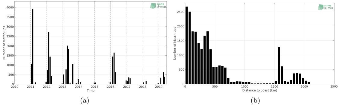
Figure 1: Number of match-ups between TSG (Polarstern) and SMOS L3 v2 - 9-Days (BEC) SSS as a function of time (a) and as function of the distance to coast (b) over the Southern Ocean Pi-MEP region and for the full satellite product period.
