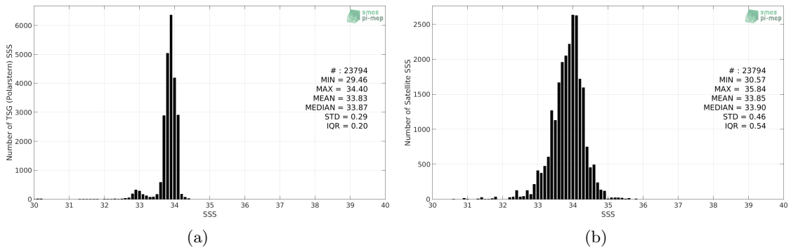
Figure 2: Histograms of SSS from TSG (Polarstern) (a) and SMOS L3 v2 - 9-Days (BEC) (b) considering all match-up pairs per bins of 0.1 over the Southern Ocean Pi-MEP region and for the full satellite product period.
