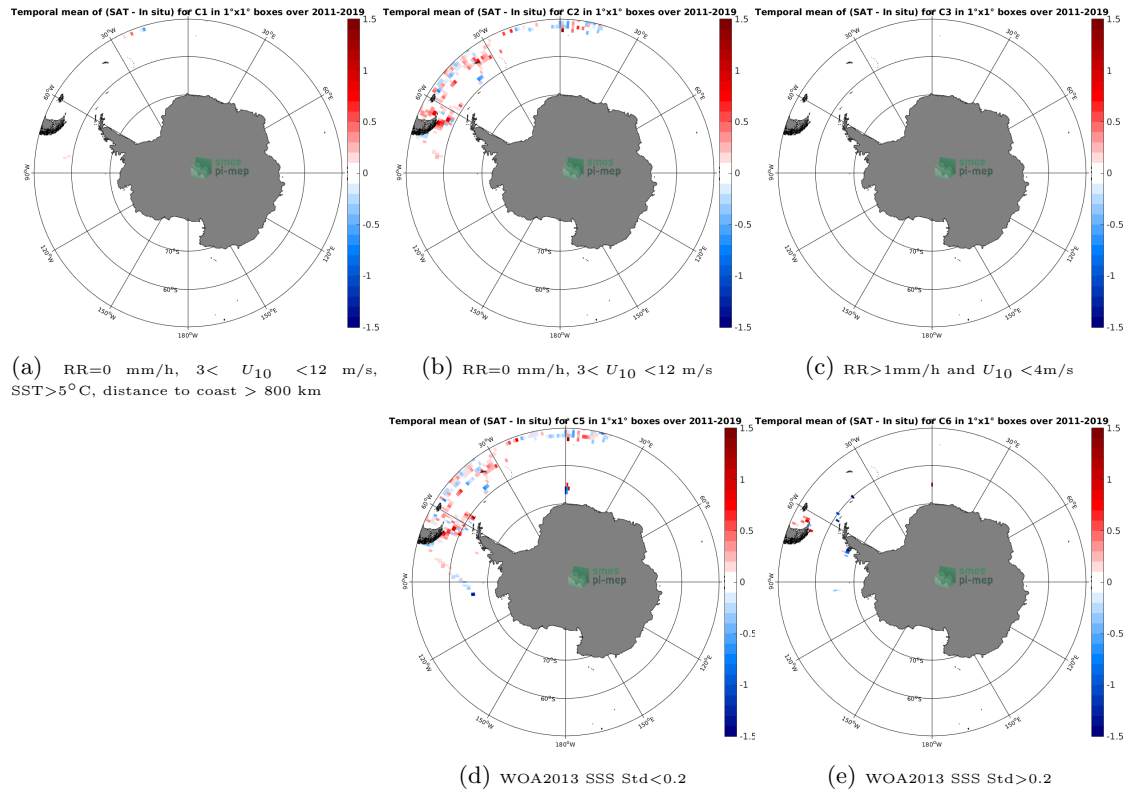
Figure 12: Temporal mean gridded over spatial boxes of size 1^{\circ}\times 1^{\circ} of \Delta\text{SSS} (SMOS L3 v2 - 9-Days (BEC) - TSG (Polarstern)) for 5 different subdatasets corresponding to:RR=0 mm/h, 3 < U_{10} < 12 m/s, SST >5^{\circ}\text{C} , distance to coast > 800 km (a), RR=0 mm/h, 3 < U_{10} < 12 m/s (b), RR >1 mm/h and U_{10} < 4 m/s (c), WOA2013 SSS Std <0.2 (d), WOA2013 SSS Std >0.2 (e).
