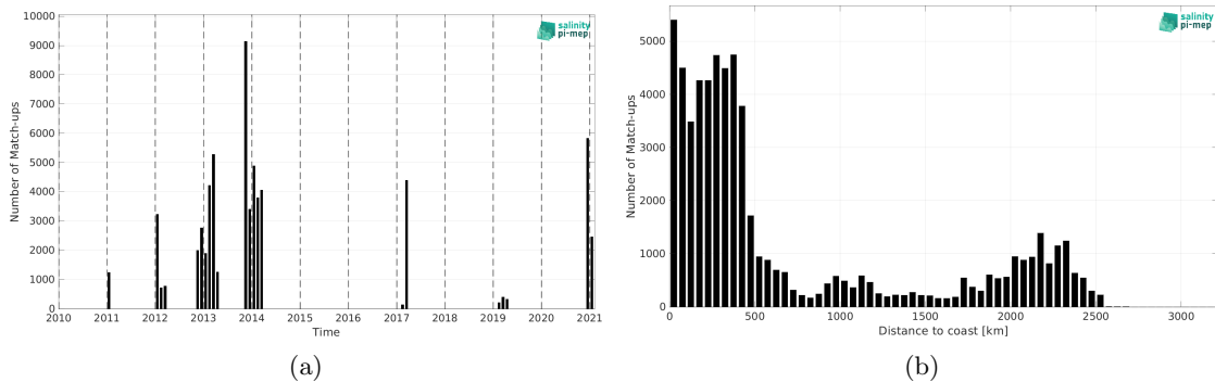
Figure 2: Number of match-ups between TSG (GOSUD-Sailing-ship) and SMOS SSS L3 v2 - 9-Days (BEC) SSS as a function of time (a) and as function of the distance to coast (b) over the Southern Ocean Pi-MEP region and for the full satellite product period.
