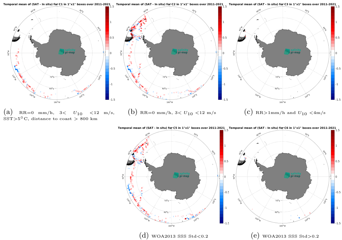
Figure 14: Temporal mean gridded over spatial boxes of size 1^\circ \times 1^\circ of \Delta\text{SSS} (SMOS SSS L3 v2 - 9-Days (BEC) - TSG (GOSUD-Sailing-ship)) for 5 different subdatasets corresponding to:RR=0 mm/h, 3 < U_{10} < 12 m/s, SST > 5^\circ\text{C} , distance to coast > 800 km (a), RR=0 mm/h, 3 < U_{10} < 12 m/s (b), RR > 1 mm/h and U_{10} < 4 m/s (c), WOA2013 SSS Std < 0.2 (d), WOA2013 SSS Std > 0.2 (e).
