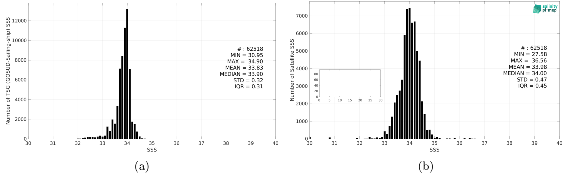
Figure 3: Histograms of SSS from TSG (GOSUD-Sailing-ship) (a) and SMOS SSS L3 v2 - 9-Days (BEC) (b) considering all match-up pairs per bins of 0.1 over the Southern Ocean Pi-MEP region and for the full satellite product period.
