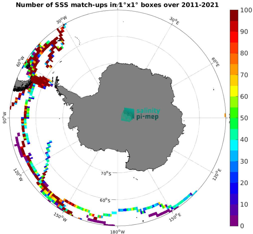
Figure 5: Number of SSS match-ups between TSG (GOSUD-Sailing-ship) SSS and the SMOS SSS L3 v2 - 9-Days (BEC) SSS product for the Southern Ocean Pi-MEP region over 1^\circ \times 1^\circ boxes and for the full satellite product period.
