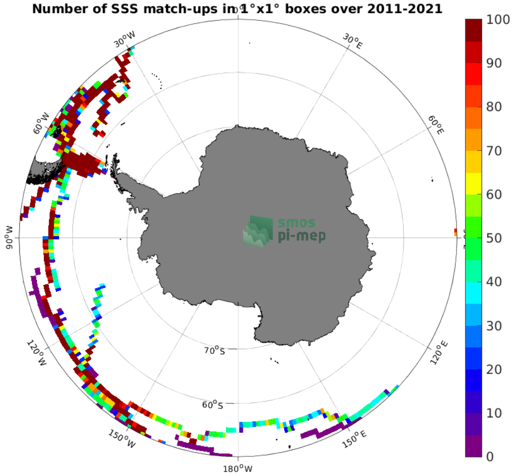
Figure 4: Number of SSS match-ups between TSG (GOSUD-Sailing-ship) SSS and the SMOS SSS L3 v2 - 9-Days (BEC) SSS product for the Southern Ocean Pi-MEP region over 1^\circ \times 1^\circ boxes and for the full satellite product period.
