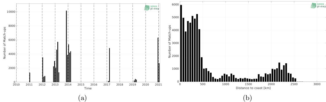
Figure 1: Number of match-ups between TSG (GOSUD-Sailing-ship) and SMOS SSS L3 v2 - 9-Days (BEC) SSS as a function of time (a) and as function of the distance to coast (b) over the Southern Ocean Pi-MEP region and for the full satellite product period.
