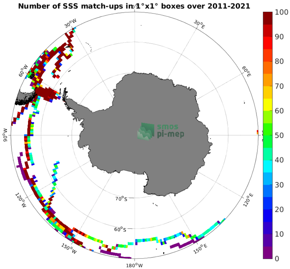
Figure 4: Number of SSS match-ups between TSG (GOSUD-Sailing-ship) SSS and the SMOS SSS L3 v2 - 9-Days (BEC) SSS product for the Southern Ocean Pi-MEP region over 1^\circ \times 1^\circ boxes and for the full satellite product period.
