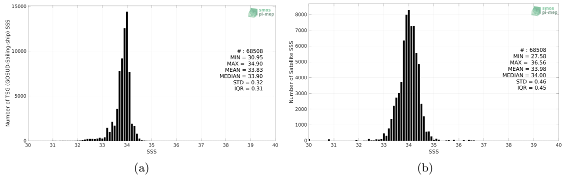
Figure 2: Histograms of SSS from TSG (GOSUD-Sailing-ship) (a) and SMOS SSS L3 v2 - 9-Days (BEC) (b) considering all match-up pairs per bins of 0.1 over the Southern Ocean Pi-MEP region and for the full satellite product period.
