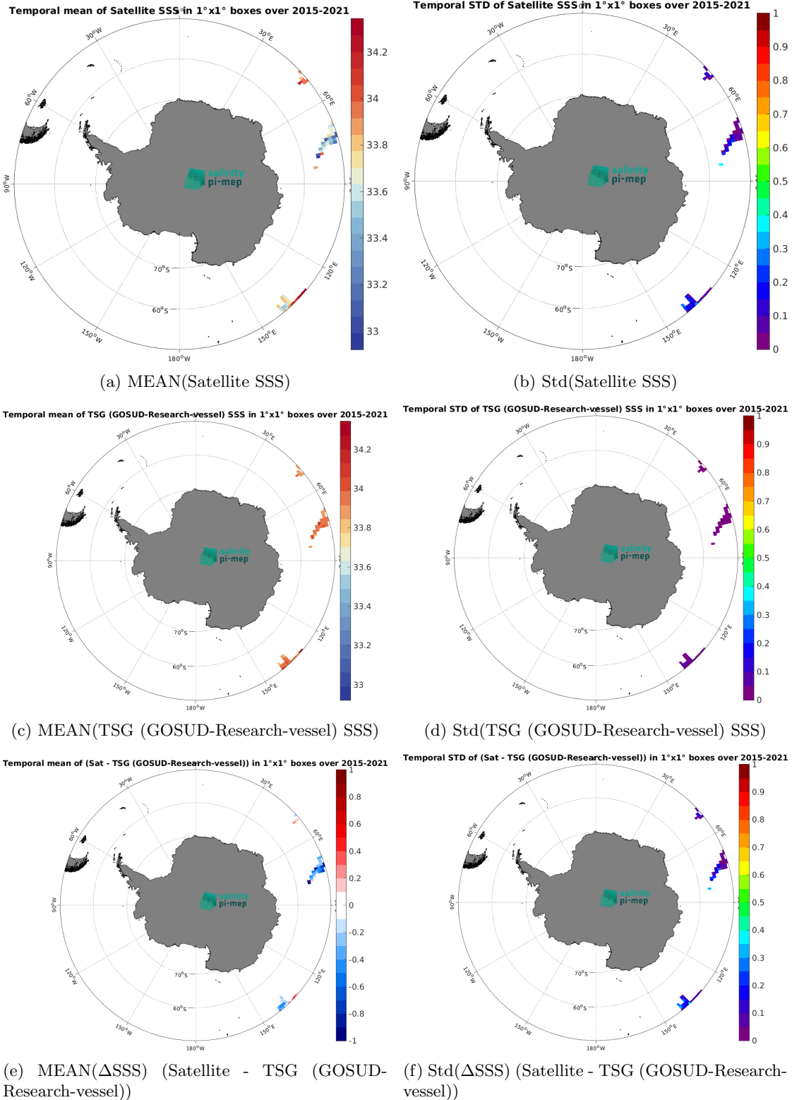
Figure 7: Temporal mean (left) and Std (right) of SSS from SMOS SSS L3 v2 - 9-Days (BEC) (top), TSG (GOSUD-Research-vessel) (middle), and of \Delta SSS (Satellite - TSG (GOSUD-Research-vessel)). Only match-up pairs are used to generate these maps.
