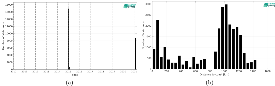
Figure 2: Number of match-ups between TSG (GOSUD-Research-vessel) and SMOS SSS L3 v2 - 9-Days (BEC) SSS as a function of time (a) and as function of the distance to coast (b) over the Southern Ocean Pi-MEP region and for the full satellite product period.
