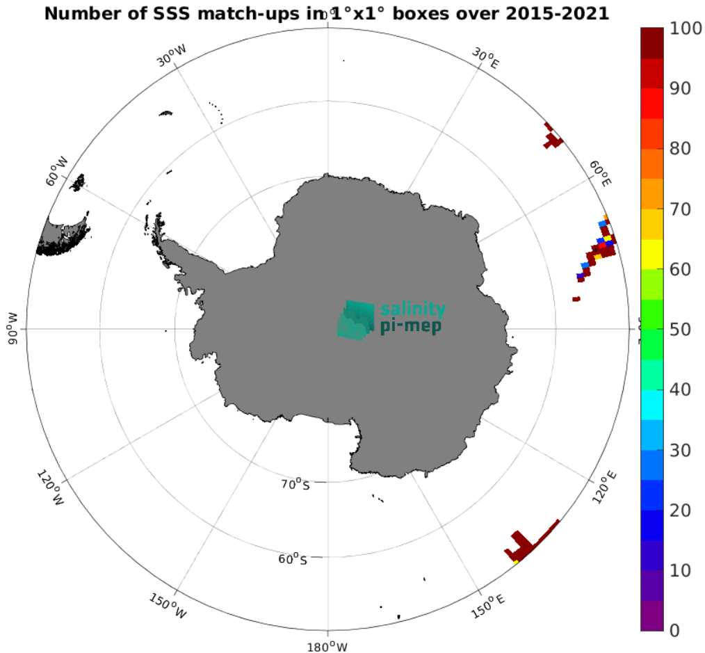
Figure 5: Number of SSS match-ups between TSG (GOSUD-Research-vessel) SSS and the SMOS SSS L3 v2 - 9-Days (BEC) SSS product for the Southern Ocean Pi-MEP region over 1^\circ \times 1^\circ boxes and for the full satellite product period.
