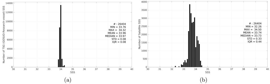
Figure 3: Histograms of SSS from TSG (GOSUD-Research-vessel) (a) and SMOS SSS L3 v2 - 9-Days (BEC) (b) considering all match-up pairs per bins of 0.1 over the Southern Ocean Pi-MEP region and for the full satellite product period.
