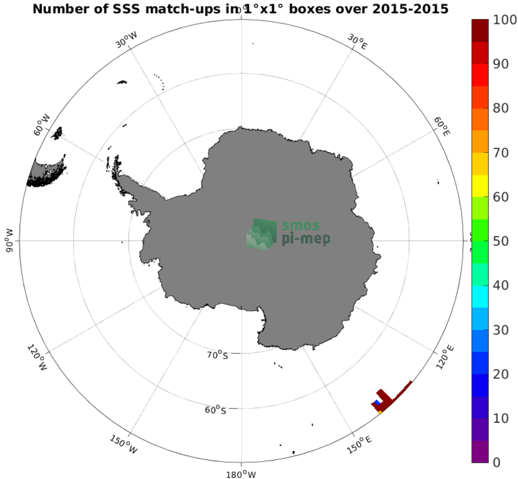
Figure 4: Number of SSS match-ups between TSG (GOSUD-Research-vessel) SSS and the SMOS SSS L3 v2 - 9-Days (BEC) SSS product for the Southern Ocean Pi-MEP region over 1^\circ \times 1^\circ boxes and for the full satellite product period.
