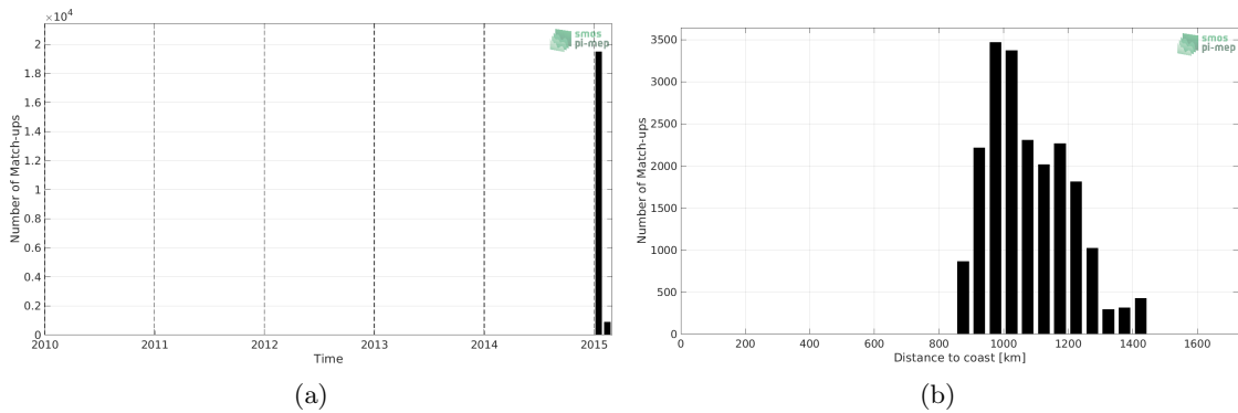
Figure 1: Number of match-ups between TSG (GOSUD-Research-vessel) and SMOS SSS L3 v2 - 9-Days (BEC) SSS as a function of time (a) and as function of the distance to coast (b) over the Southern Ocean Pi-MEP region and for the full satellite product period.
