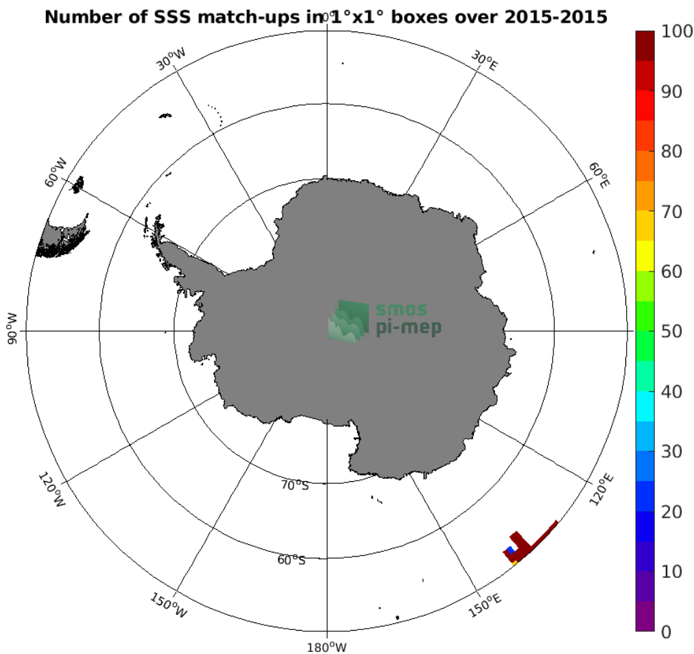
Figure 4: Number of SSS match-ups between TSG (GOSUD-Research-vessel) SSS and the SMOS SSS L3 v2 - 9-Days (BEC) SSS product for the Southern Ocean Pi-MEP region over 1^\circ \times 1^\circ boxes and for the full satellite product period.
