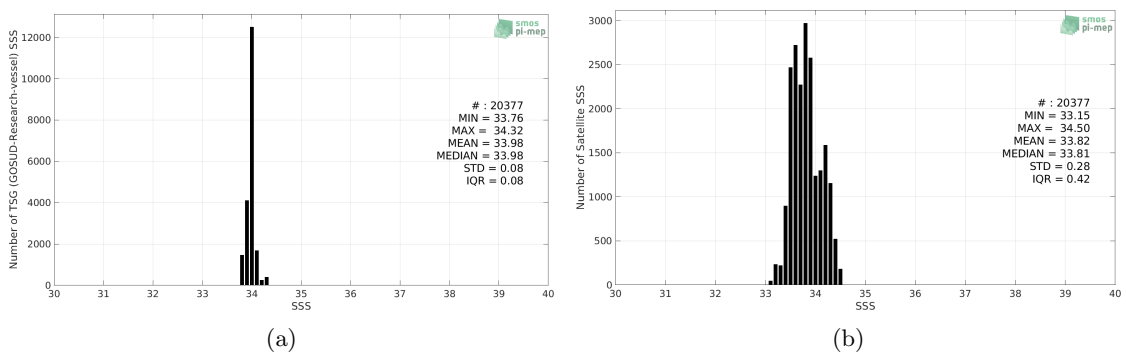
Figure 2: Histograms of SSS from TSG (GOSUD-Research-vessel) (a) and SMOS SSS L3 v2 - 9-Days (BEC) (b) considering all match-up pairs per bins of 0.1 over the Southern Ocean Pi-MEP region and for the full satellite product period.
