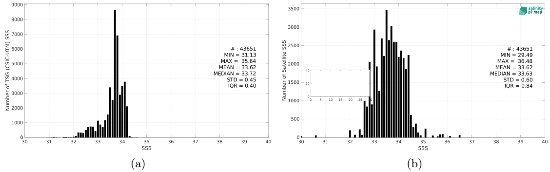
Figure 3: Histograms of SSS from TSG (CSIC-UTM) (a) and SMOS SSS L3 v2 - 9-Days (BEC) (b) considering all match-up pairs per bins of 0.1 over the Southern Ocean Pi-MEP region and for the full satellite product period.
