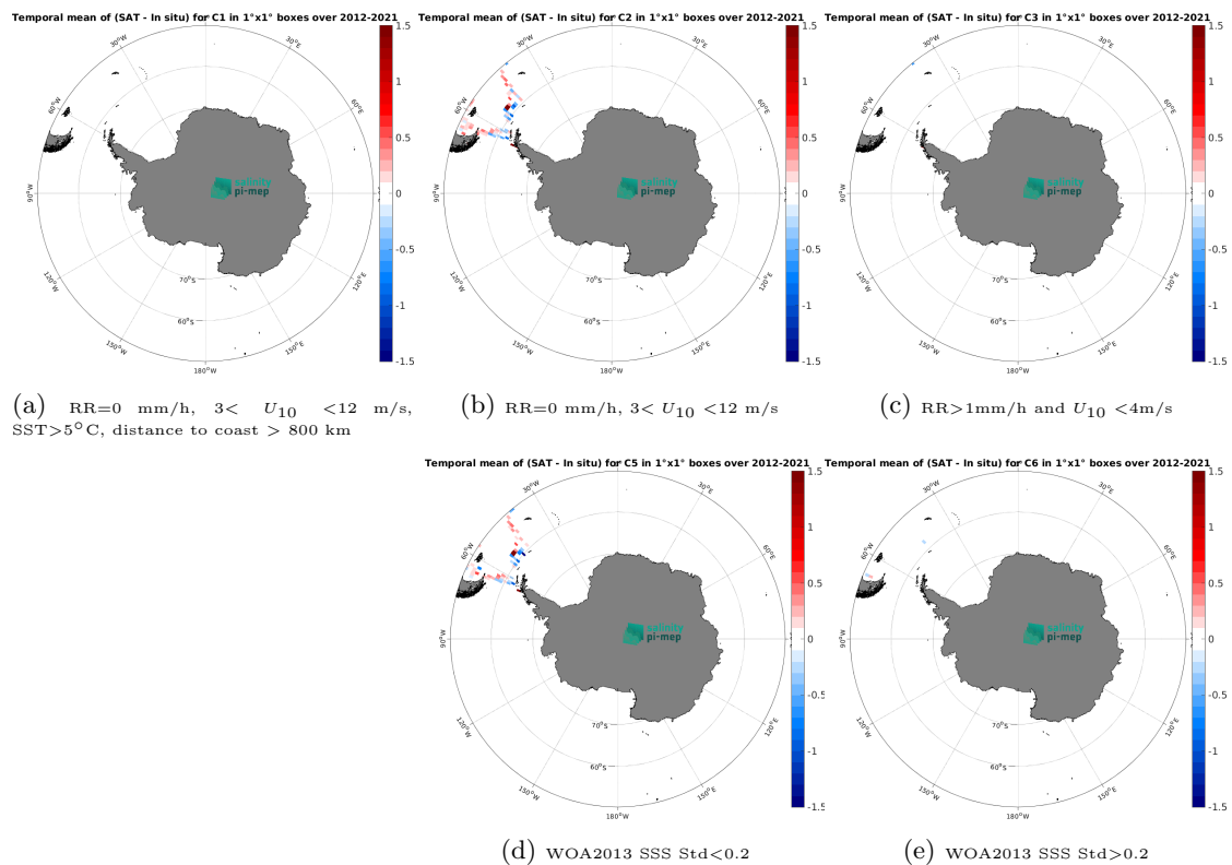
Figure 14: Temporal mean gridded over spatial boxes of size 1^\circ \times 1^\circ of \Delta\text{SSS} (SMOS SSS L3 v2 - 9-Days (BEC) - TSG (CSIC-UTM)) for 5 different subdatasets corresponding to:RR=0 mm/h, 3 < U_{10} < 12 m/s, SST>5°C, distance to coast > 800 km (a), RR=0 mm/h, 3 < U_{10} < 12 m/s (b), RR>1mm/h and U_{10} < 4 m/s (c), WOA2013 SSS Std<0.2 (d), WOA2013 SSS Std>0.2 (e).
