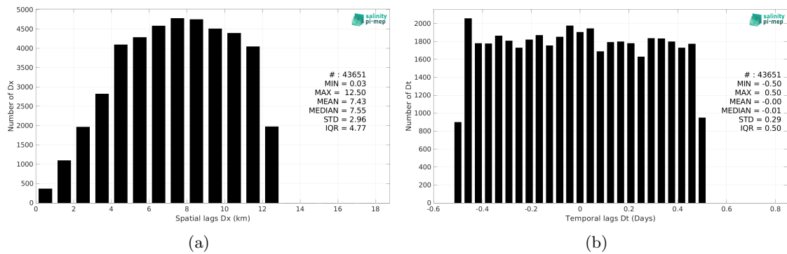
Figure 6: Histograms of the spatial (a) and temporal (b) lags between the location/time of the TSG (CSIC-UTM) measurement and the date of the corresponding SMOS SSS L3 v2 - 9-Days (BEC) SSS pixel.
