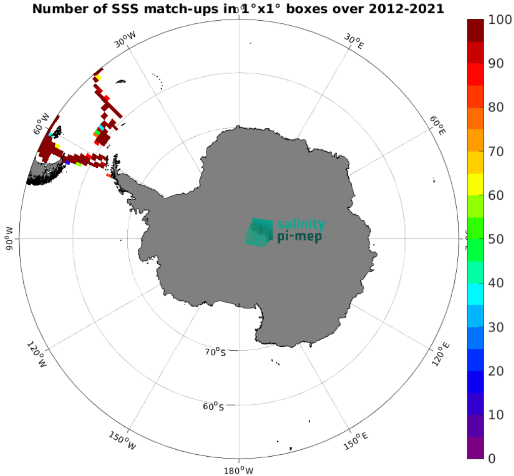
Figure 5: Number of SSS match-ups between TSG (CSIC-UTM) SSS and the SMOS SSS L3 v2 - 9-Days (BEC) SSS product for the Southern Ocean Pi-MEP region over 1^\circ \times 1^\circ boxes and for the full satellite product period.
