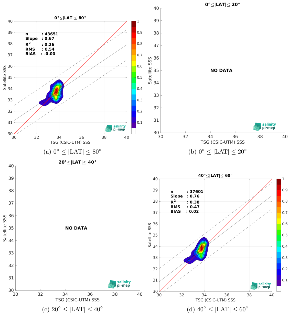
Figure 10: Contour maps of the concentration of SMOS SSS L3 v2 - 9-Days (BEC) SSS (y-axis) versus TSG (CSIC-UTM) SSS (x-axis) at match-up pairs for different latitude bands. For each plot, the red line shows x=y . The black thin and dashed lines indicate a linear fit through the data cloud and the \pm 95\% confidence levels, respectively. The number match-up pairs n , the slope and R^2 coefficient of the linear fit, the root mean square (RMS) and the mean bias between satellite and in situ data are indicated for each latitude band in each plots.
