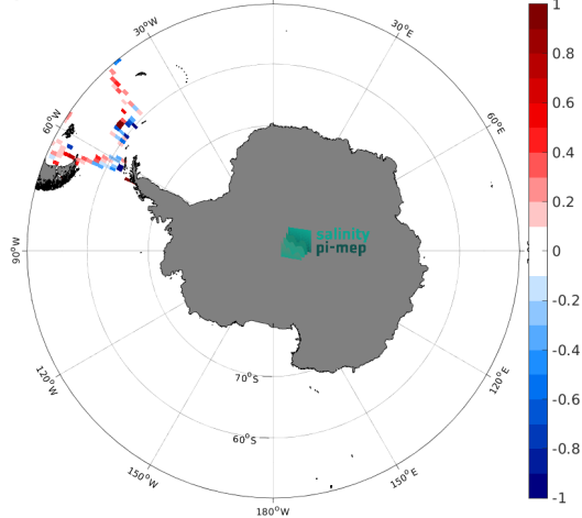
(e) MEAN( \Delta SSS) (Satellite - TSG (CSIC-UTM)) 16
