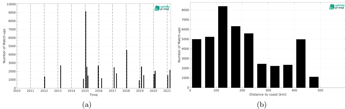
Figure 2: Number of match-ups between TSG (CSIC-UTM) and SMOS SSS L3 v2 - 9-Days (BEC) SSS as a function of time (a) and as function of the distance to coast (b) over the Southern Ocean Pi-MEP region and for the full satellite product period.
