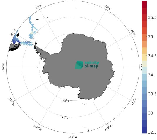
(c) MEAN(TSG (CSIC-UTM) SSS)
