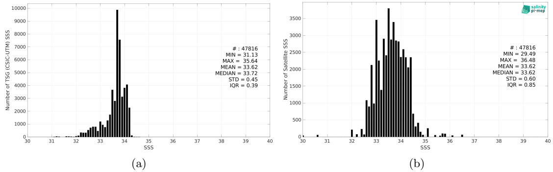
Figure 2: Histograms of SSS from TSG (CSIC-UTM) (a) and SMOS SSS L3 v2 - 9-Days (BEC) (b) considering all match-up pairs per bins of 0.1 over the Southern Ocean Pi-MEP region and for the full satellite product period.
