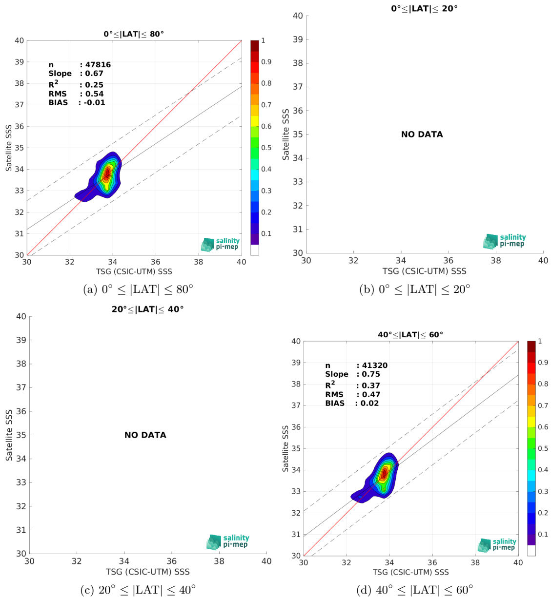
Figure 9: Contour maps of the concentration of SMOS SSS L3 v2 - 9-Days (BEC) SSS (y-axis) versus TSG (CSIC-UTM) SSS (x-axis) at match-up pairs for different latitude bands. For each plot, the red line shows x=y . The black thin and dashed lines indicate a linear fit through the data cloud and the \pm 95\% confidence levels, respectively. The number match-up pairs n , the slope and R^2 coefficient of the linear fit, the root mean square (RMS) and the mean bias between satellite and in situ data are indicated for each latitude band in each plots.
