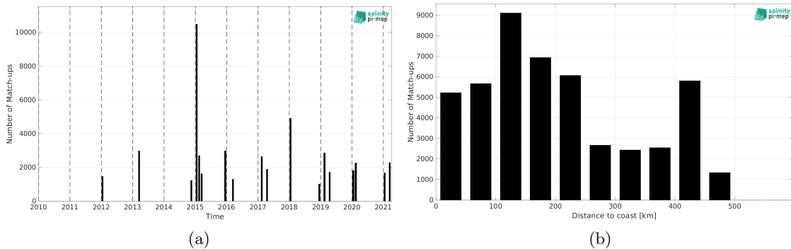
Figure 1: Number of match-ups between TSG (CSIC-UTM) and SMOS SSS L3 v2 - 9-Days (BEC) SSS as a function of time (a) and as function of the distance to coast (b) over the Southern Ocean Pi-MEP region and for the full satellite product period.
