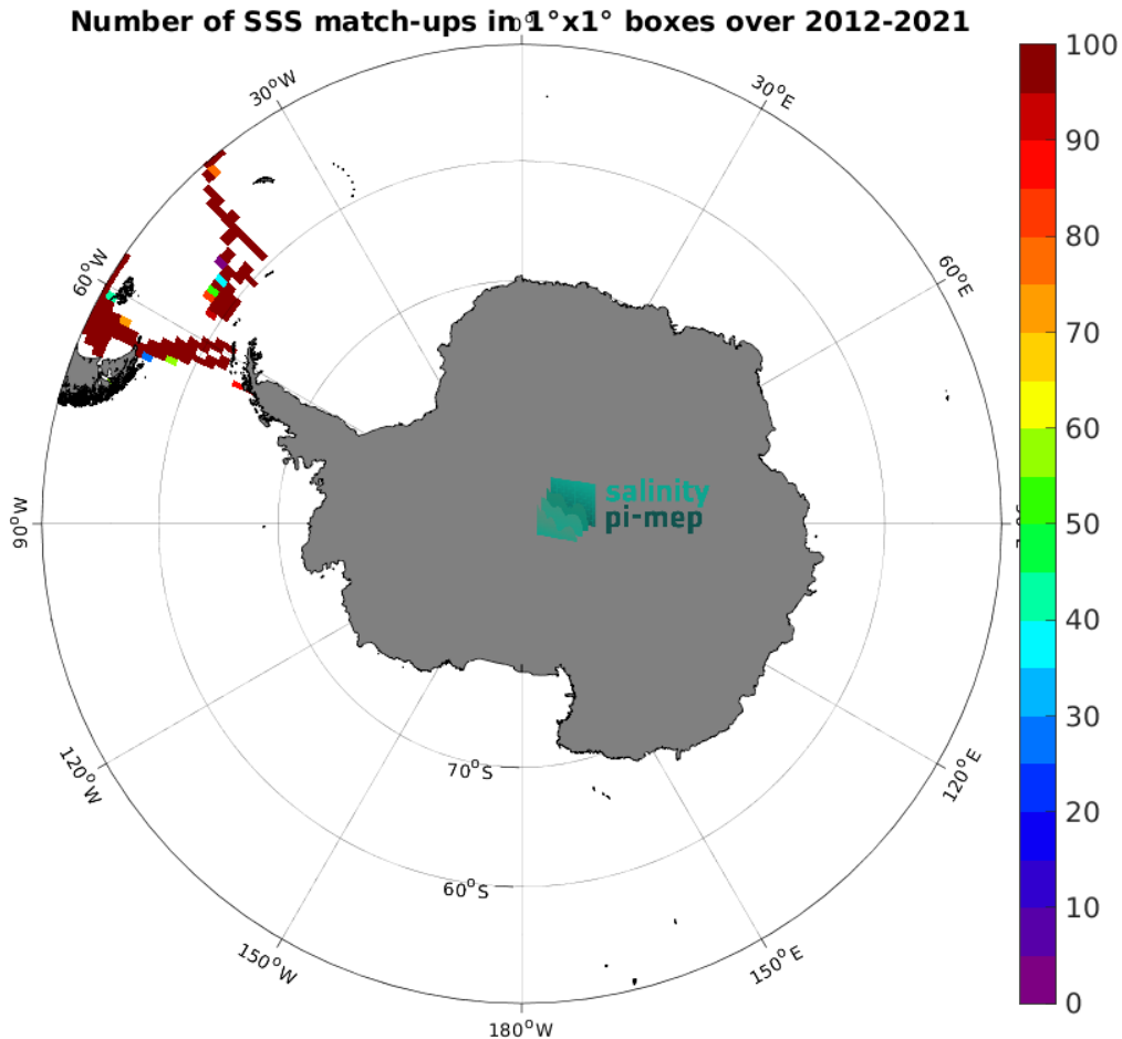
Figure 4: Number of SSS match-ups between TSG (CSIC-UTM) SSS and the SMOS SSS L3 v2 - 9-Days (BEC) SSS product for the Southern Ocean Pi-MEP region over 1^\circ \times 1^\circ boxes and for the full satellite product period.
