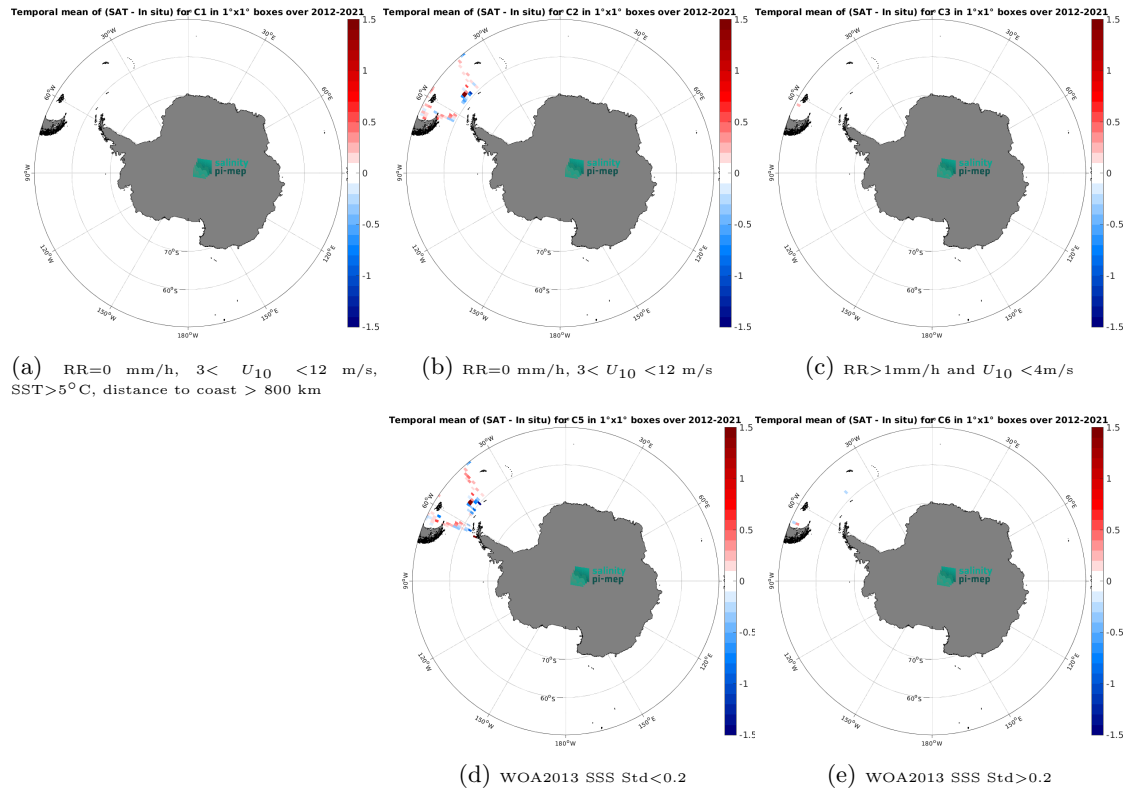
Figure 12: Temporal mean gridded over spatial boxes of size 1^{\circ}\times 1^{\circ} of \Delta\text{SSS} (SMOS SSS L3 v2 - 9-Days (BEC) - TSG (CSIC-UTM)) for 5 different subdatasets corresponding to: \text{RR}=0 mm/h, 3 < U_{10} < 12 m/s, \text{SST}>5^{\circ}\text{C} , distance to coast > 800 km (a), \text{RR}=0 mm/h, 3 < U_{10} < 12 m/s (b), \text{RR}>1 mm/h and U_{10} < 4 m/s (c), WOA2013 SSS Std < 0.2 (d), WOA2013 SSS Std > 0.2 (e).
