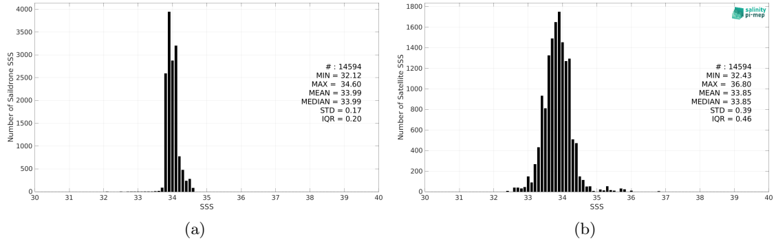
Figure 2: Histograms of SSS from Saildrone (a) and SMOS SSS L3 v2 - 9-Days (BEC) (b) considering all match-up pairs per bins of 0.1 over the Southern Ocean Pi-MEP region and for the full satellite product period.
