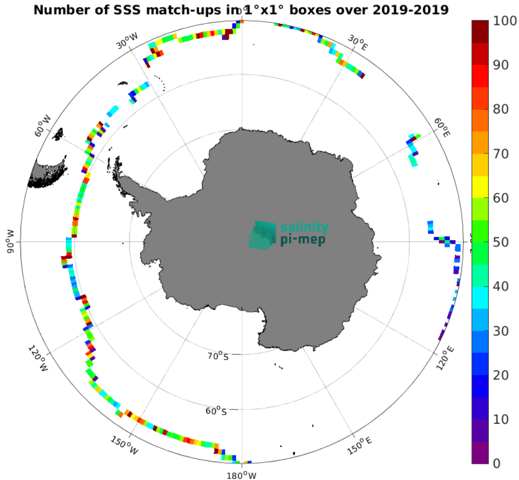
Figure 4: Number of SSS match-ups between Saildrone SSS and the SMOS SSS L3 v2 - 9-Days (BEC) SSS product for the Southern Ocean Pi-MEP region over 1^\circ \times 1^\circ boxes and for the full satellite product period.
