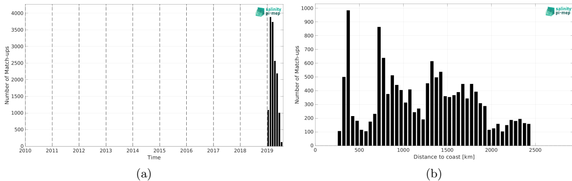
Figure 1: Number of match-ups between Saildrone and SMOS SSS L3 v2 - 9-Days (BEC) SSS as a function of time (a) and as function of the distance to coast (b) over the Southern Ocean Pi-MEP region and for the full satellite product period.
