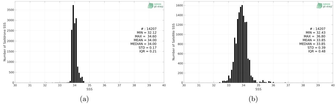
Figure 2: Histograms of SSS from Sairdrone (a) and SMOS SSS L3 v2 - 9-Days (BEC) (b) considering all match-up pairs per bins of 0.1 over the Southern Ocean Pi-MEP region and for the full satellite product period.
