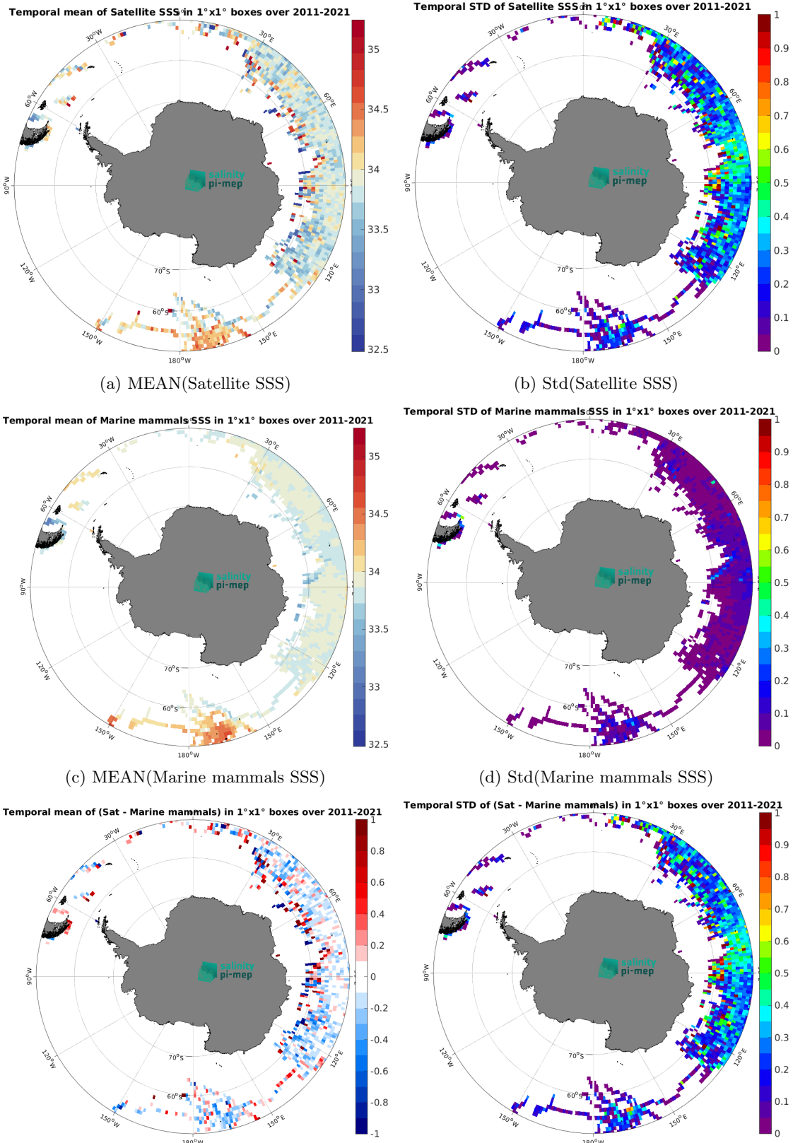
Figure 7: Temporal mean (left) and Std (right) of SSS from SMOS SSS L3 v2 - 9-Days (BEC) (top), Marine mammals (middle), and of \Delta SSS (Satellite - Marine mammals). Only match-up pairs are used to generate these maps.
