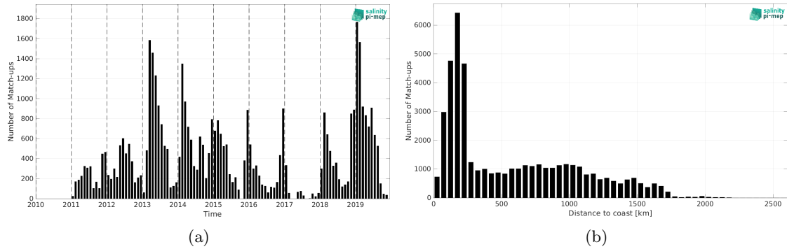
Figure 1: Number of match-ups between Marine mammals and SMOS SSS L3 v2 - 9-Days (BEC) SSS as a function of time (a) and as function of the distance to coast (b) over the Southern Ocean Pi-MEP region and for the full satellite product period.
