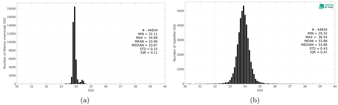
Figure 2: Histograms of SSS from Marine mammals (a) and SMOS SSS L3 v2 - 9-Days (BEC) (b) considering all match-up pairs per bins of 0.1 over the Southern Ocean Pi-MEP region and for the full satellite product period.
