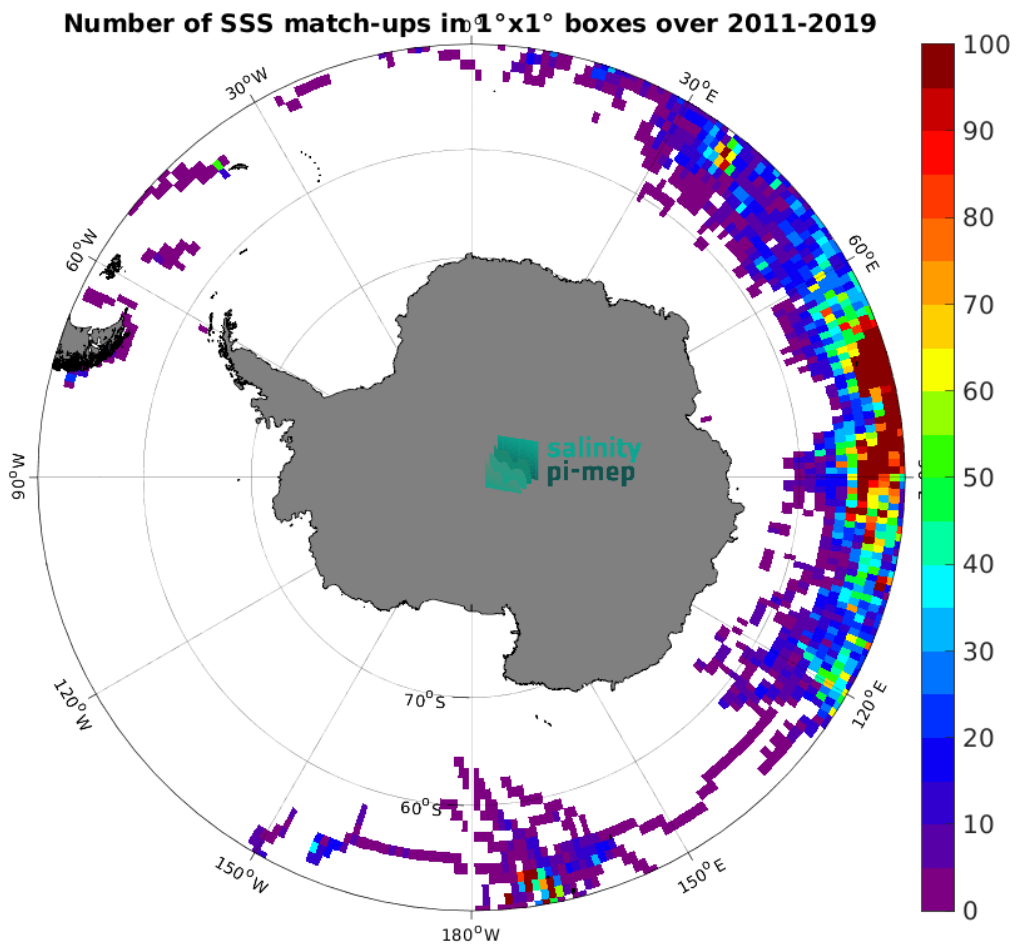
Figure 4: Number of SSS match-ups between Marine mammals SSS and the SMOS SSS L3 v2 - 9-Days (BEC) SSS product for the Southern Ocean Pi-MEP region over 1^\circ \times 1^\circ boxes and for the full satellite product period.
